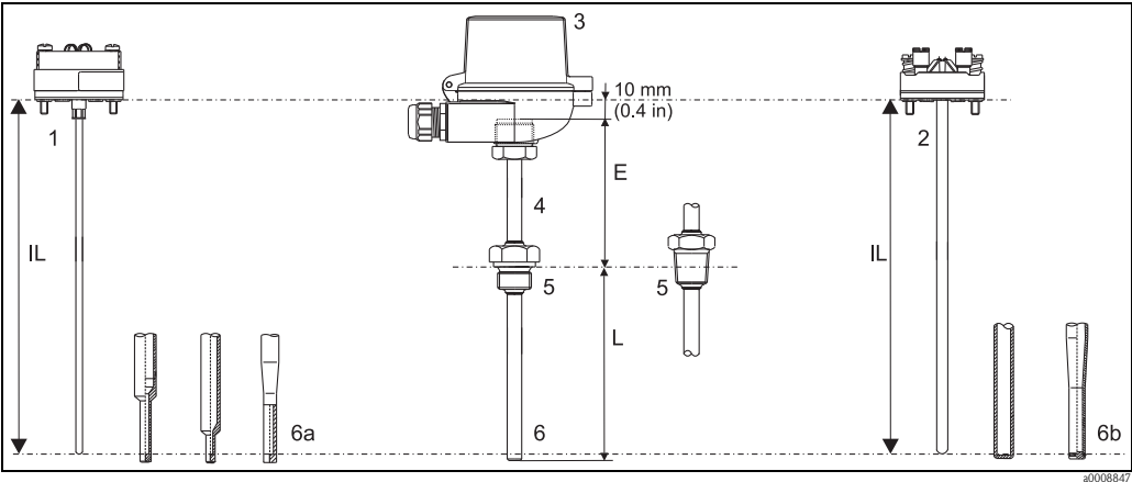
Equipment architecture of the Omnigrad M TR10
