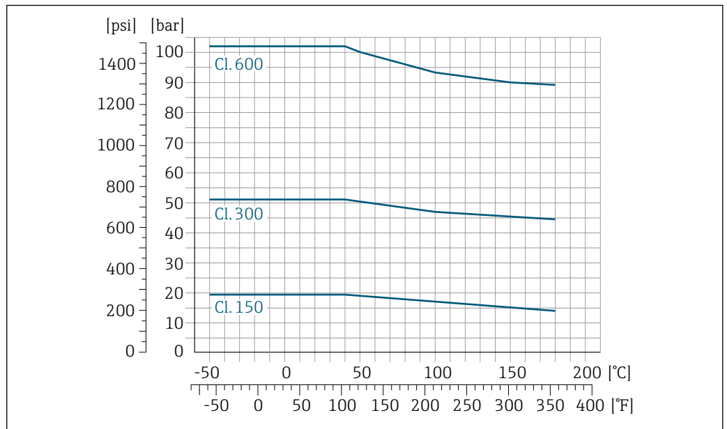
23 Com material de flange 1.4404 (316/316L)
