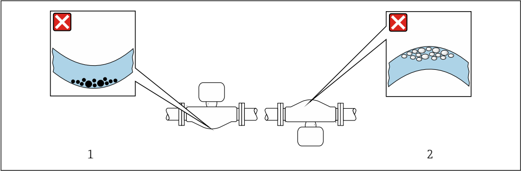
14 Orientation of sensor with curved measuring tube 1 Avoid this orientation for media with entrained solids: Risk of solids accumulating 2 Avoid this orientation for outgassing media: Risk of gas accumulating
