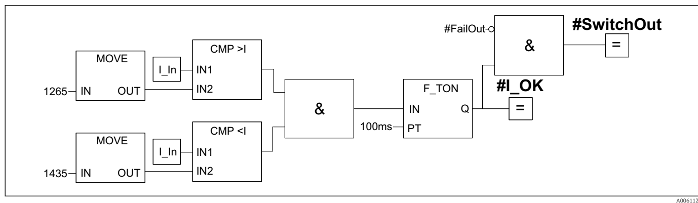
27 Function block, switch output
