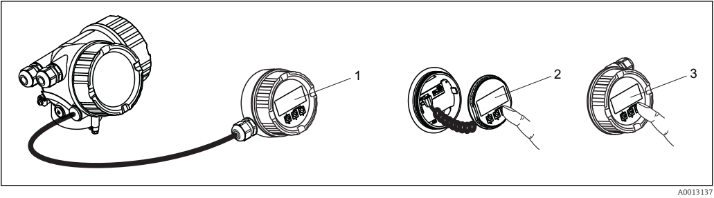
16 FHX50 operating options
