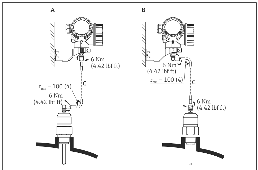
12 Connecting the cable. There are the following possibilities:
