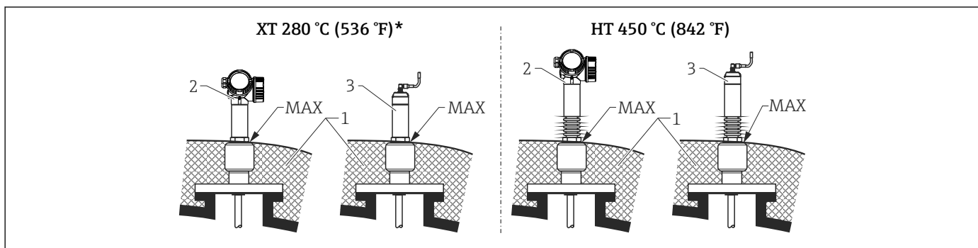
10 Process connection with flange - FMP54, sensor version XT and HT
