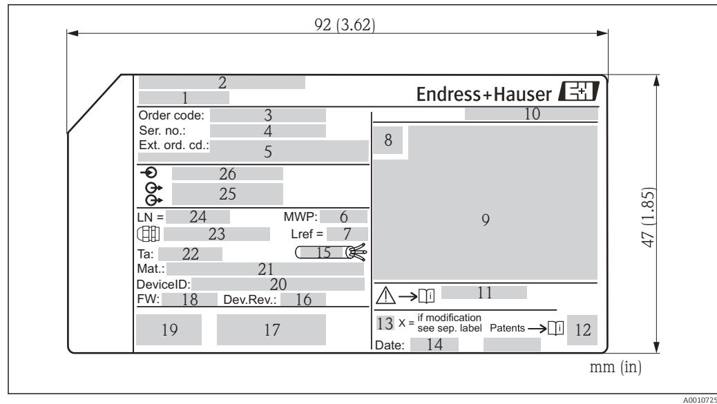
3 Nameplate of the Levelflex
