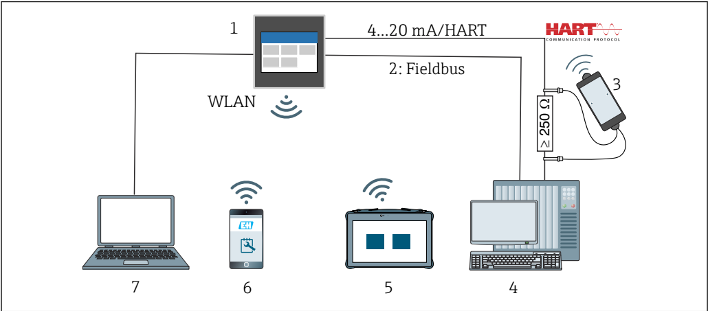
30 Systemintegration
