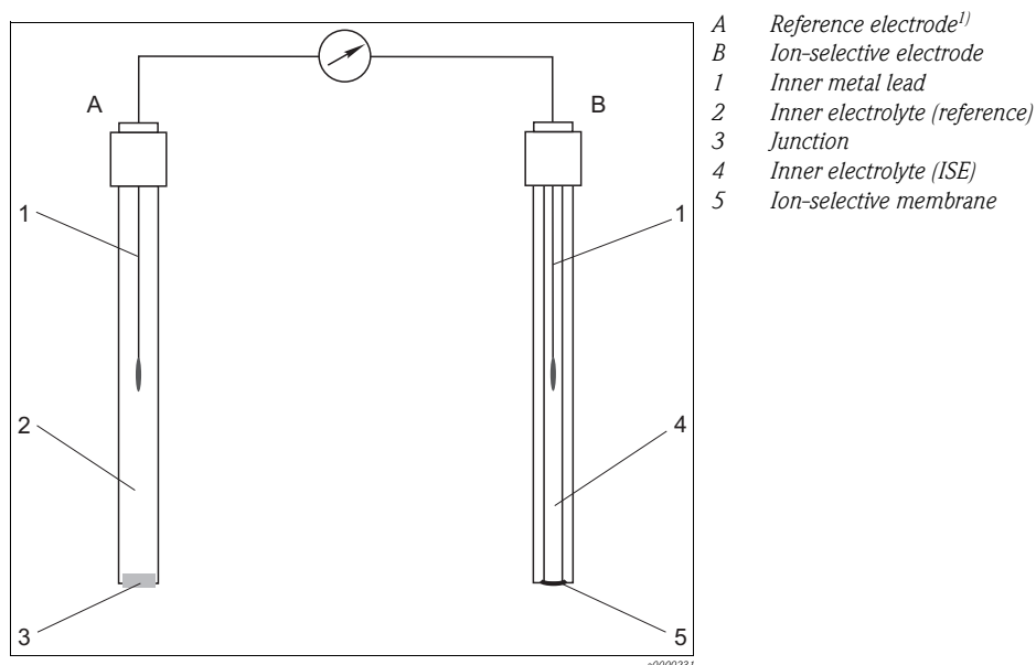
General measuring principle of an ion-selective electrode
