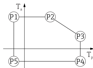
42 Custodia 316L; temperatura di processo -40 \dots +280 \text{ }^{\circ}\text{C} ( -40 \dots +536 \text{ }^{\circ}\text{F} )
