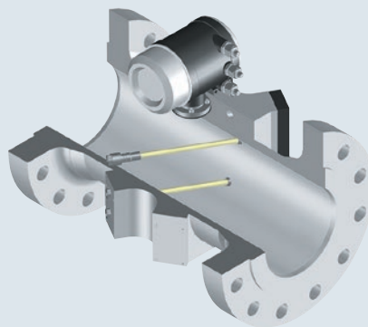
FLOWSIC600, 2-path
