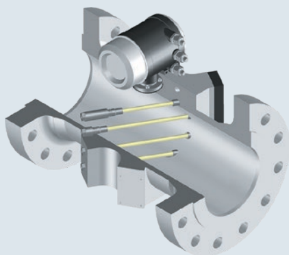
FLOWSIC600, 4-path
