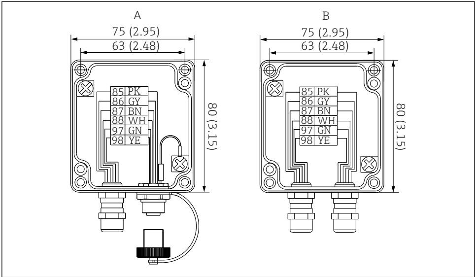
2 Versions of CYK11 junction box. Engineering unit: mm (in)
