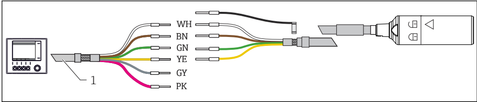
9 Electrical connection, CYK11 as extension for CYK10
