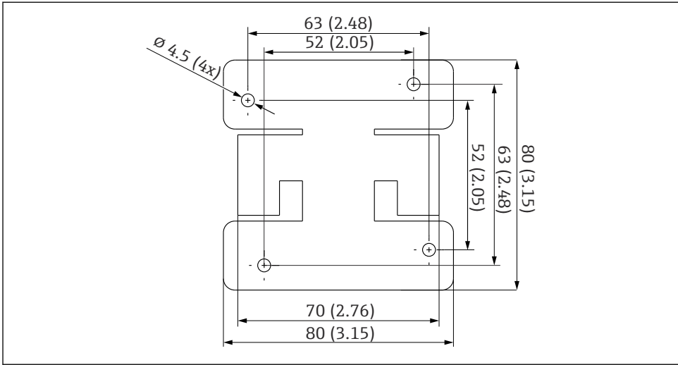
3 Securing plate. Engineering unit: mm (in)
