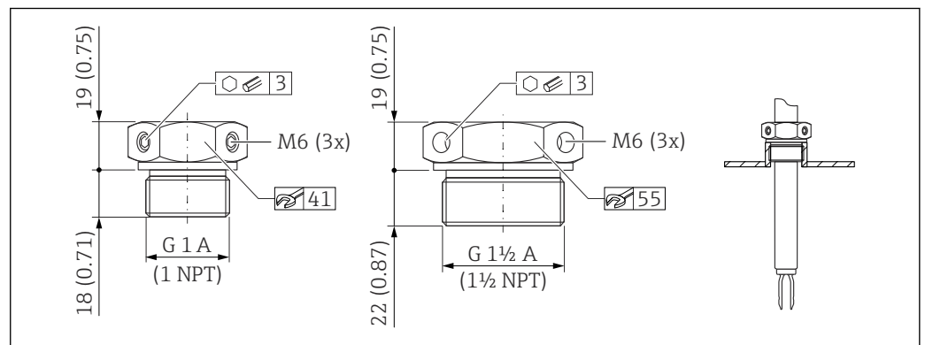
66 Sliding sleeves for unpressurized operation p_e = 0 bar (0 psi). Unit of measurement mm (in)
