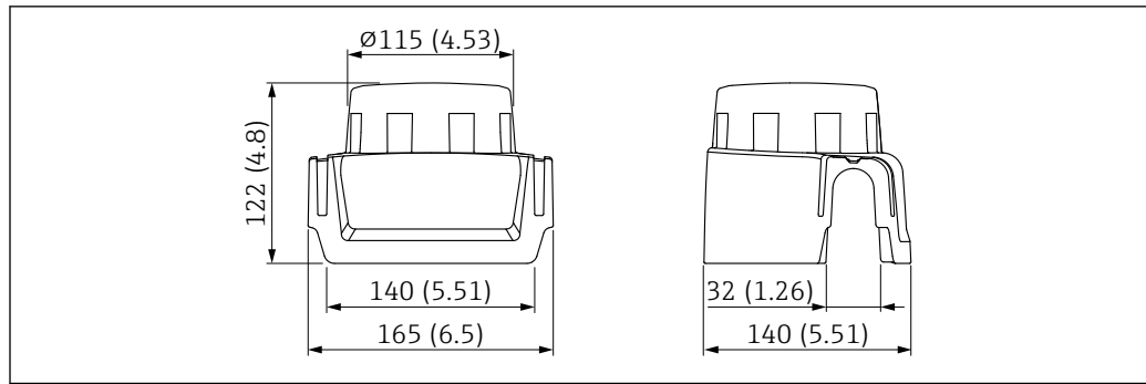
63 Dimensions of protective cover, plastic, XW111. Unit of measurement mm (in)
