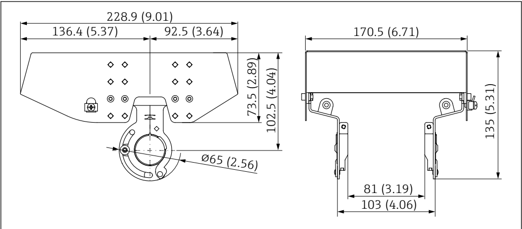
62 Dimensions of protective cover, 316 L, XW112. Unit of measurement mm (in)
