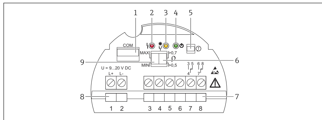
55 Example of electronic insert FEL64DC
