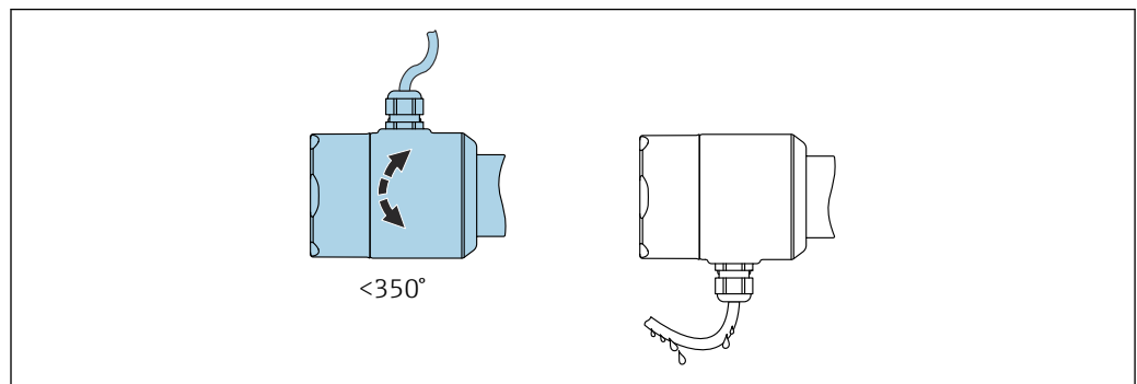
26 Housing without set screw; form a drip loop on the cable.
