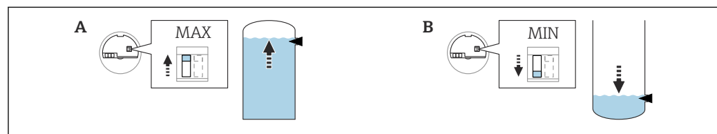
56 Switch position on the electronic insert for MAX/MIN safety mode
