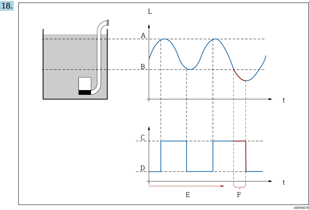
64 “Backlash interval”和“Backlash time”的影响
