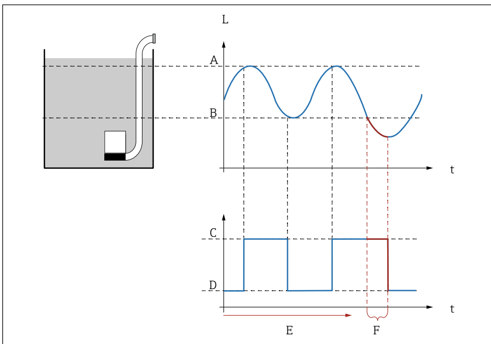
58 “Backlash interval”和“Backlash time”的影响
