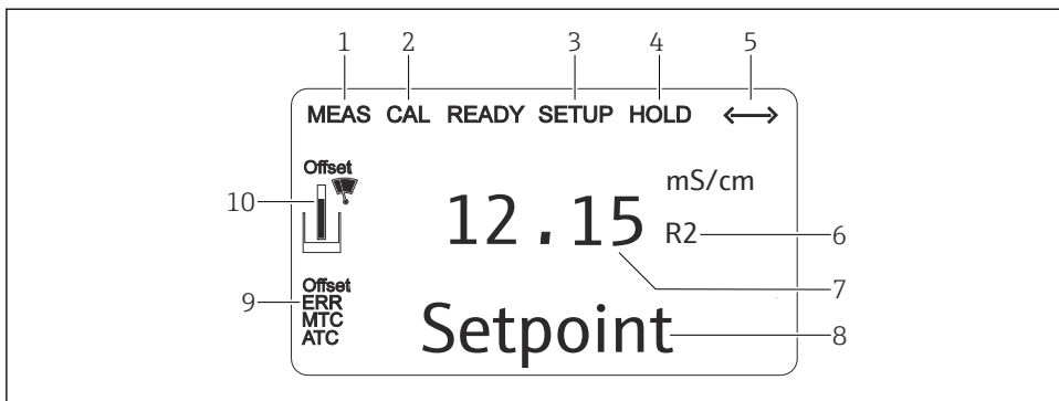
10 Transmitter LC-display
