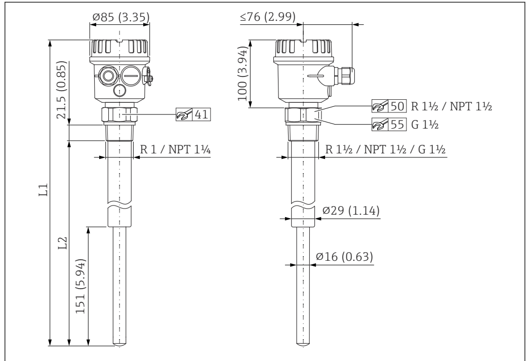
2 Threaded process connection with F16 polyester housing
