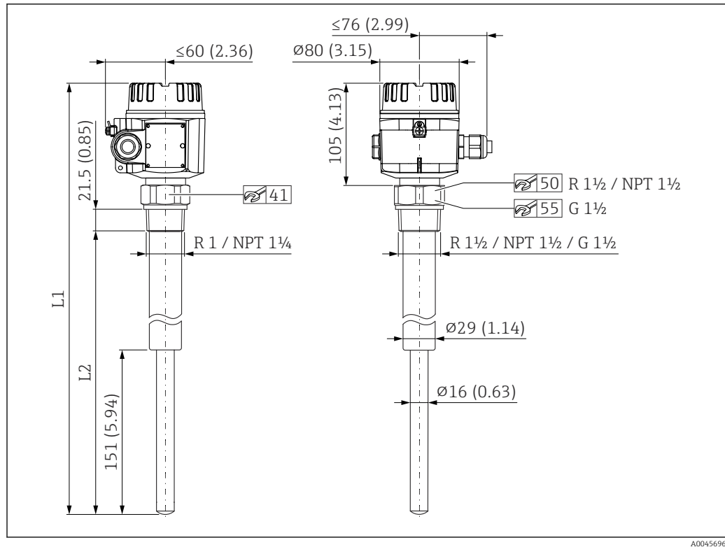
3 Threaded process connection with F18 aluminum housing
