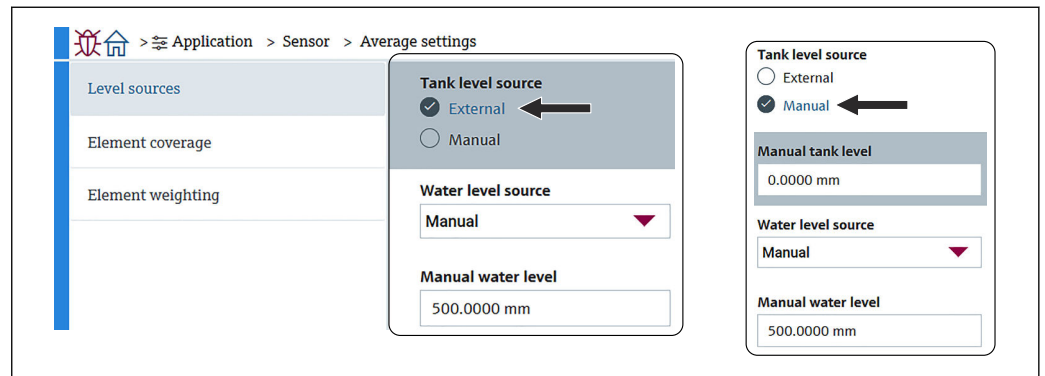
81 Экран Tank level source / Water level source
