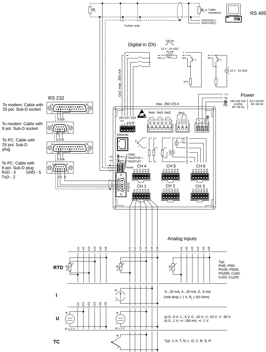
Fig. 4: Wiring diagram
