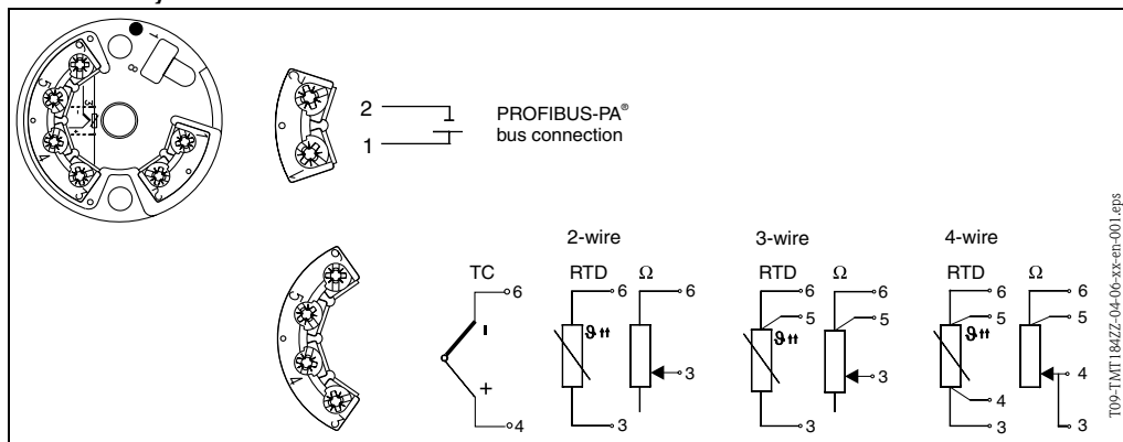
fig. 5: Head transmitter wiring
