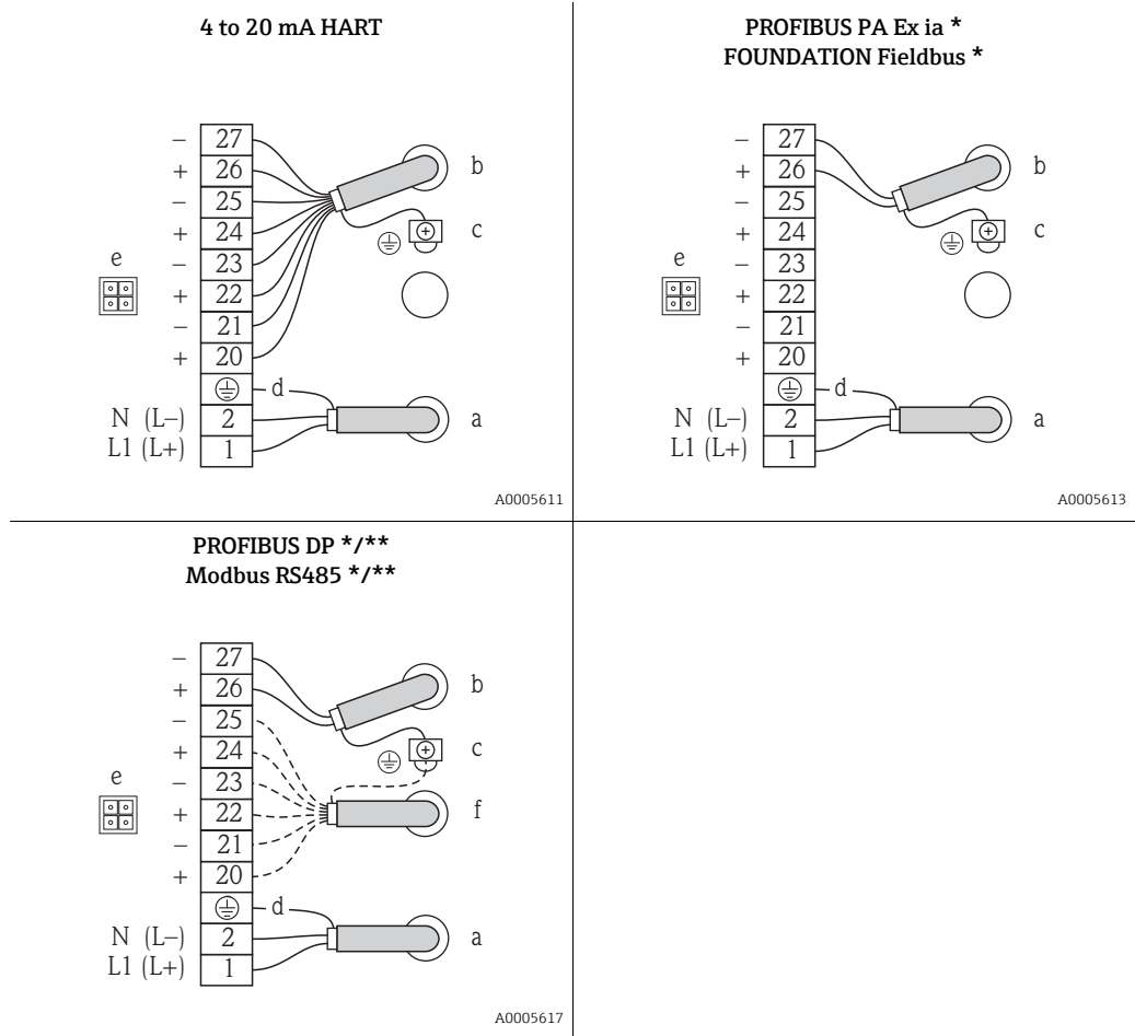
Fig. 7: Electrical connections
