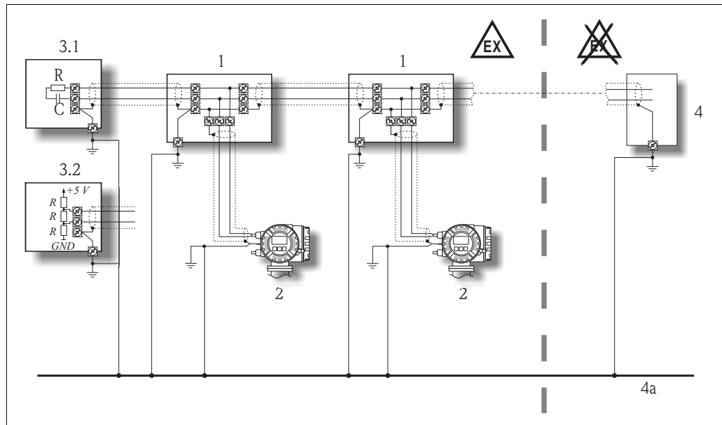
Fig. 5: Example for connecting potential equalization lines
