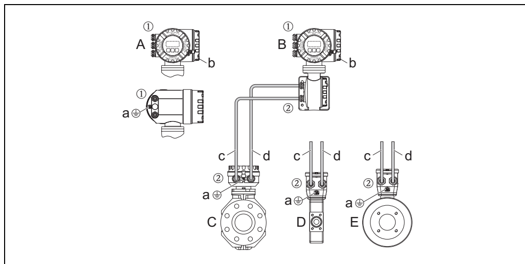
Fig. 4: Design of the measuring system, compact/remote version
