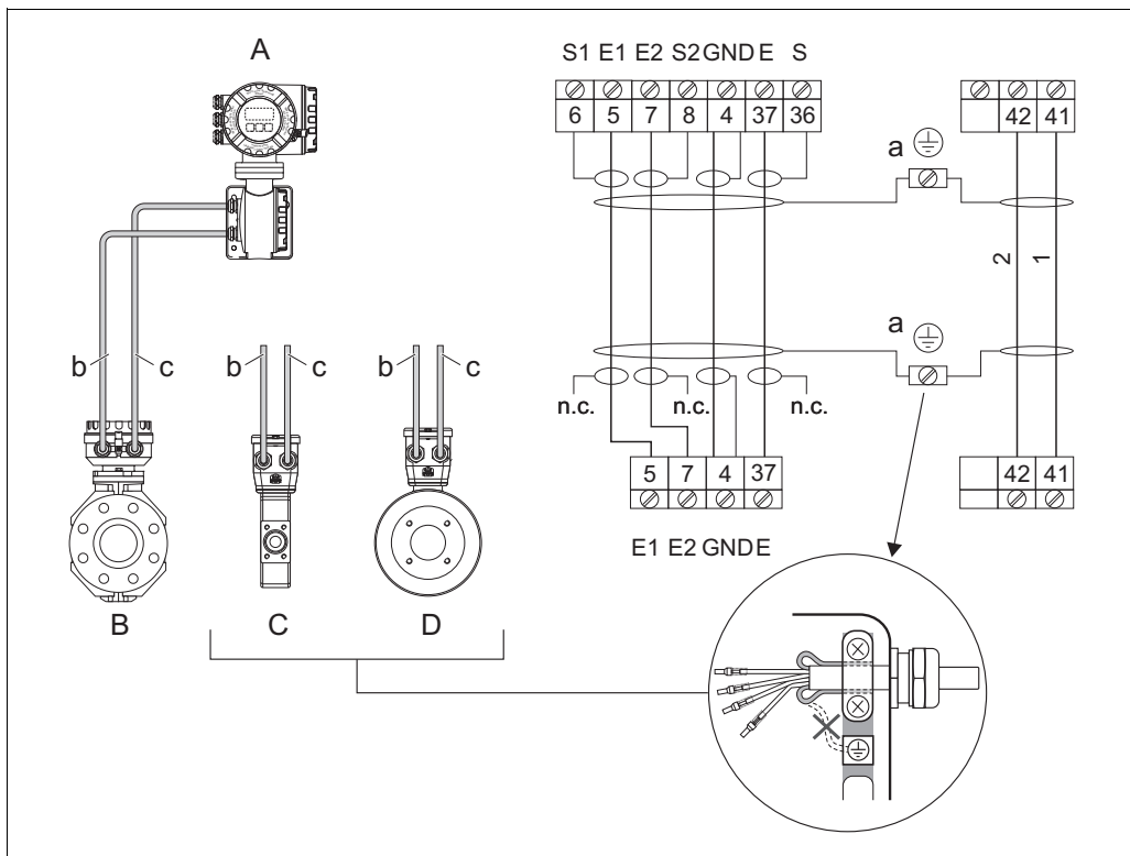
Fig. 6: Connection of remote version connecting cable
