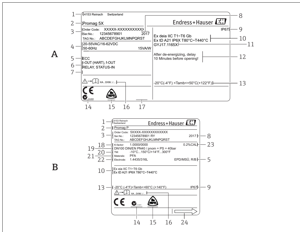
Fig. 2: Example for nameplates of a transmitter and of a sensor, compact version
