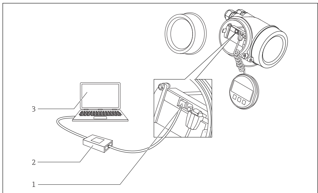
19 DeviceCare/FieldCare via interface service (CDI)
