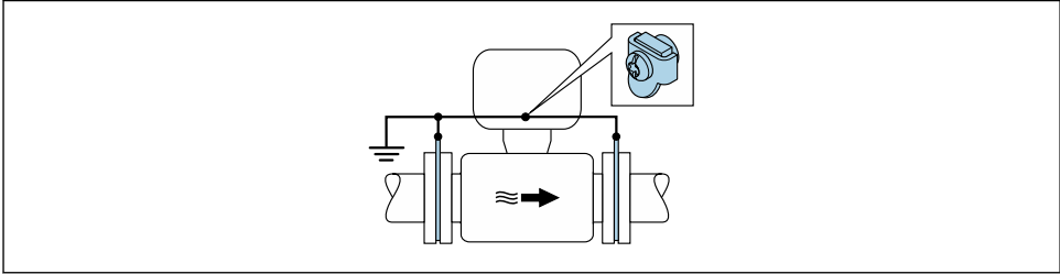
3 Potential equalization via ground terminal and ground disks
