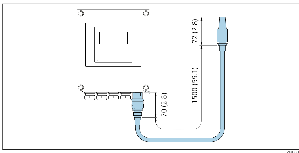
46 Engineering unit mm (in)
