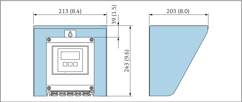
43 Weather protection cover for Proline 500 – digital
