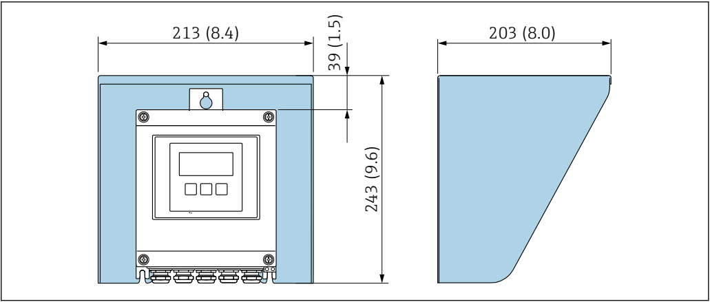
37 Weather protection cover for Proline 500 – digital
