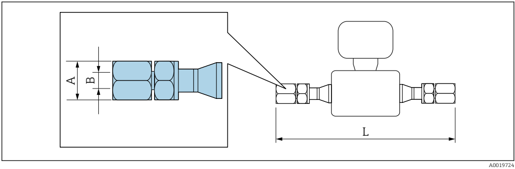
Adapter, NPT to 4-VCO-4
