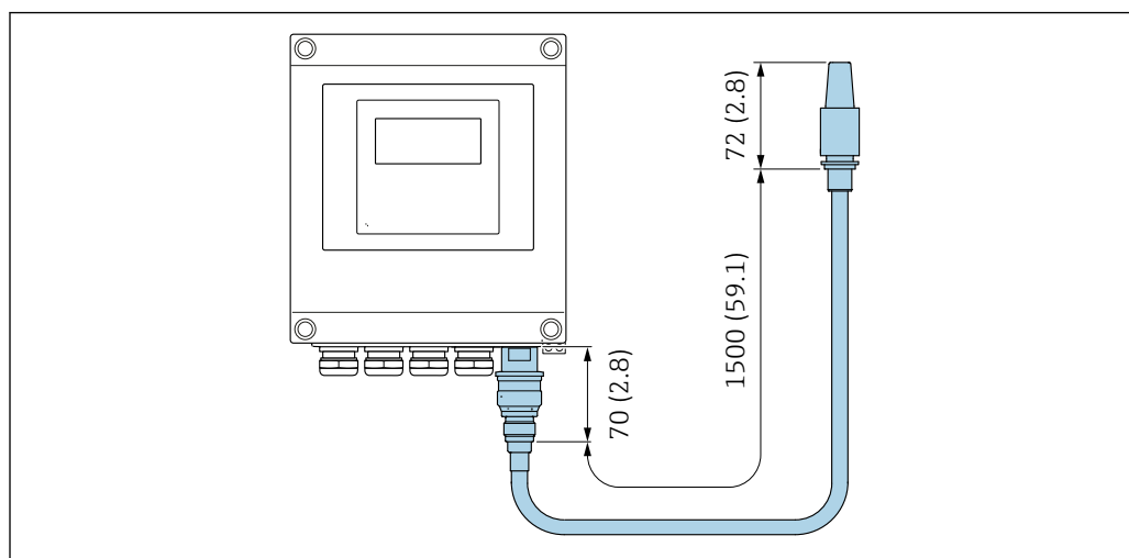
40 Engineering unit mm (in)
