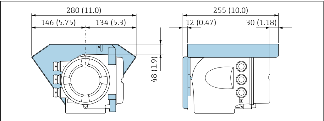
38 Weather protection cover for Proline 500
