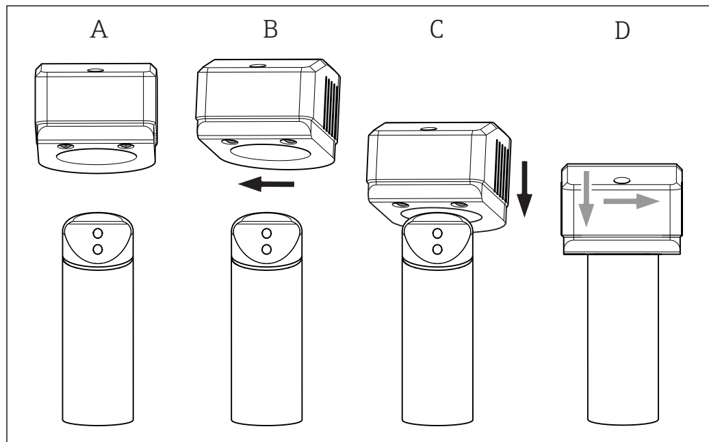
36 Fitting the solid state reference on the sensor
