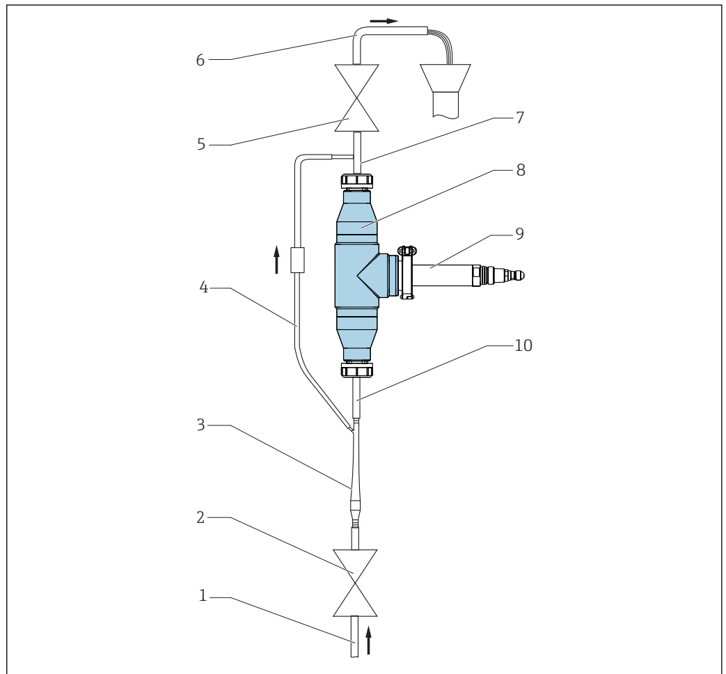
21 Connection example with bubble trap and CUA252 flow assembly
