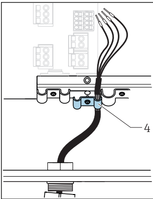
26 Inserting the cable
