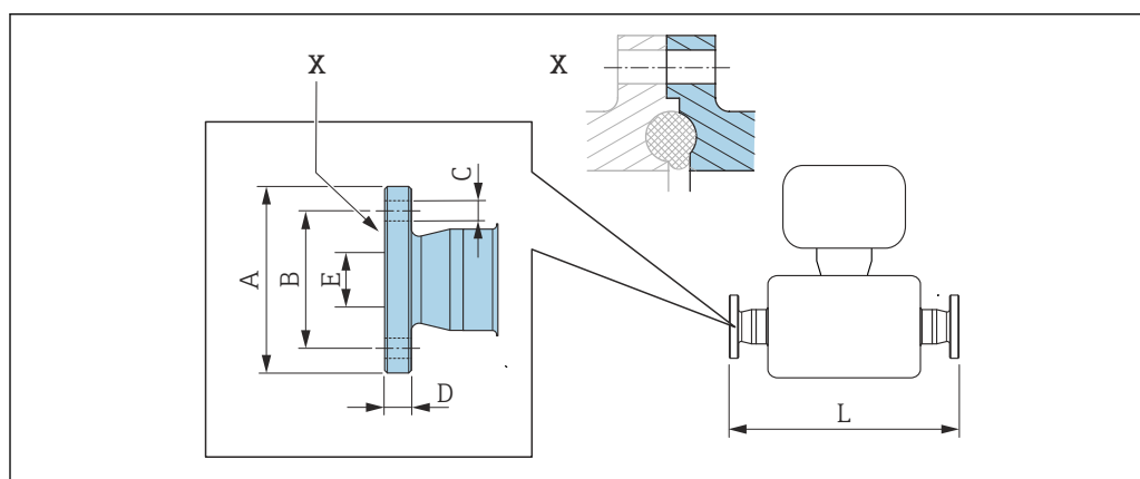
32 Detail X: Asymmetrical process connection; the part shown in gray is provided by the supplier.
