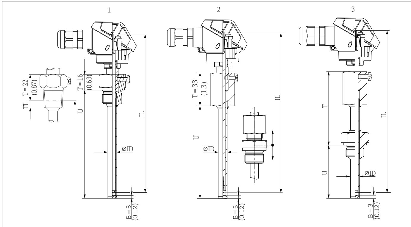
10 Thermometer design with Mignon head
