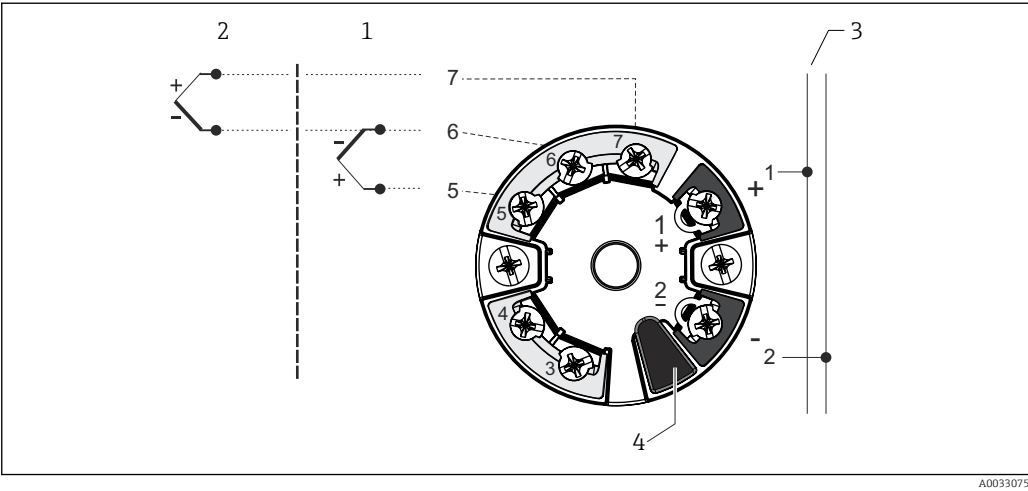
2 Wiring diagram of the dual sensor input head transmitters (TMT8x)
