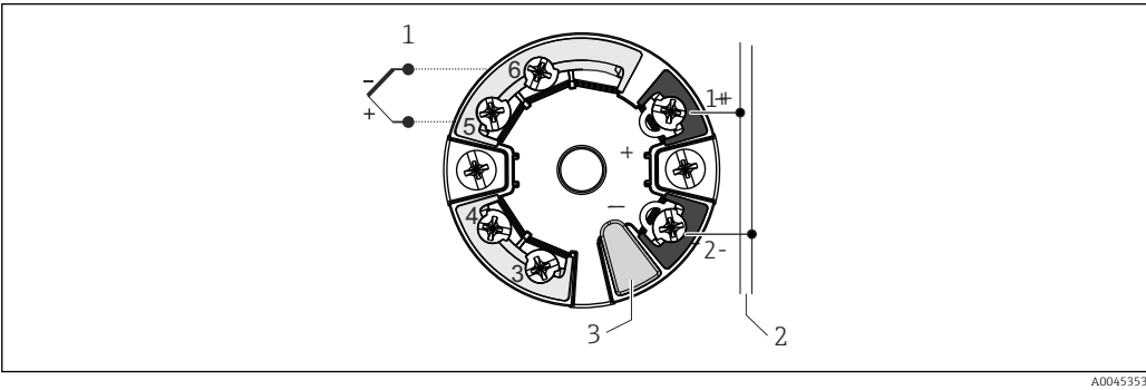
3 Wiring diagram of the single input head transmitters (TMT7x)
