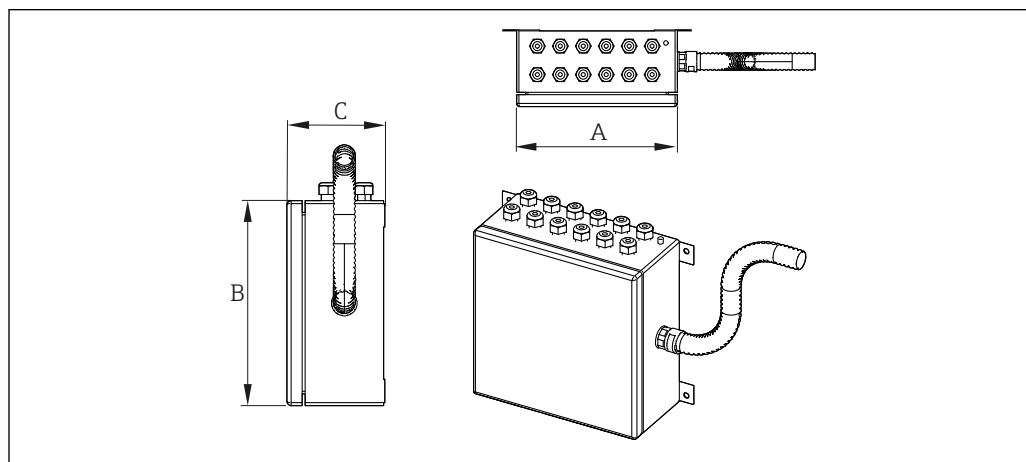
6 Junction box as accessory for remote installation
