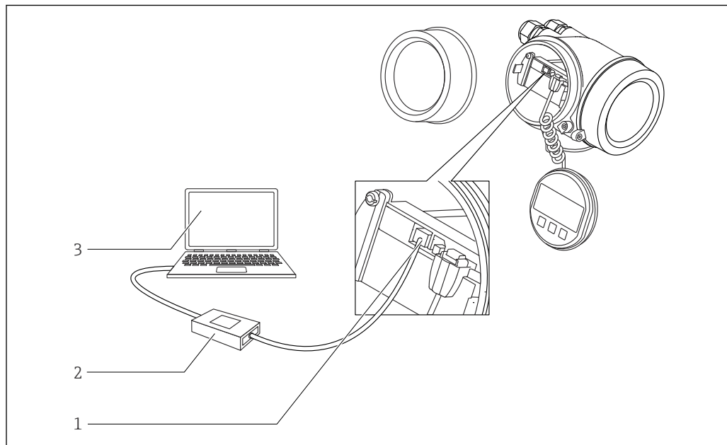
20 DeviceCare/FieldCare mediante interfaccia service (CDI)
