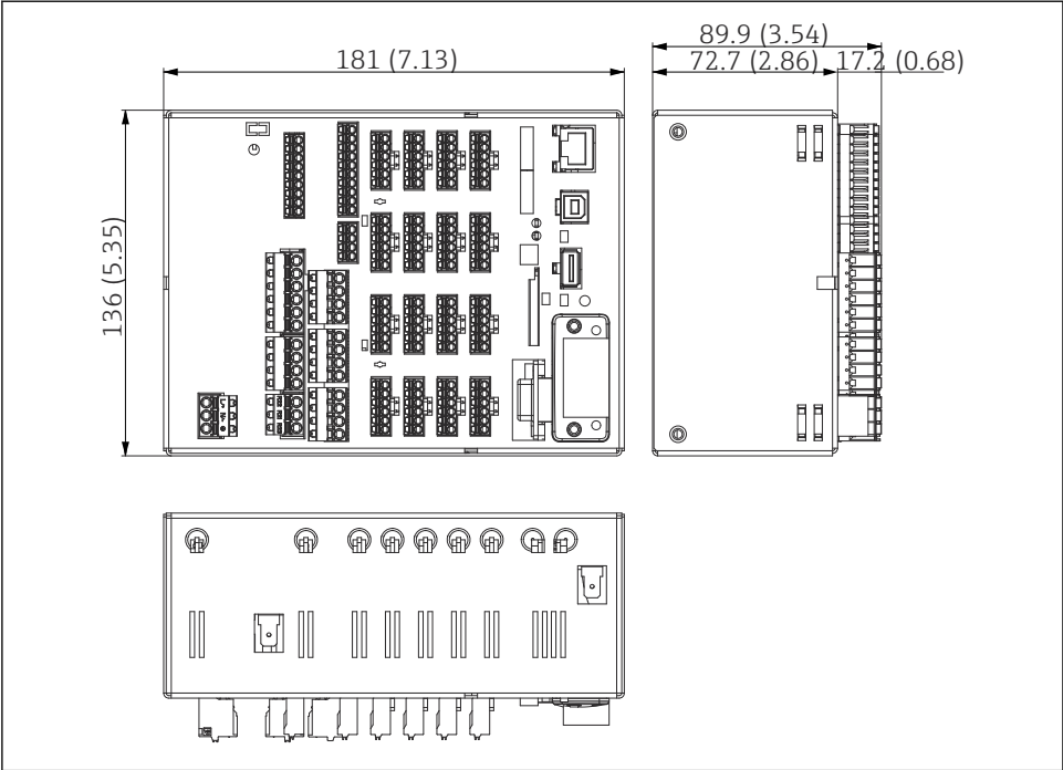
2 DIN rail Version, Maße in mm (in)
