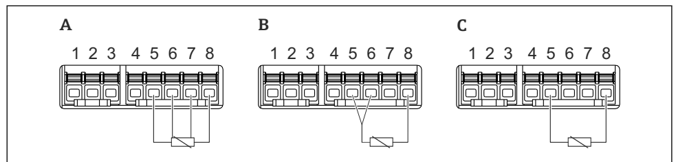
63 Types de raccordement RTD
