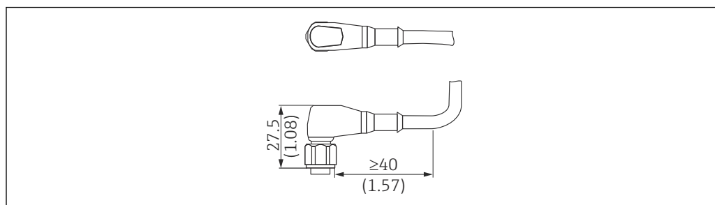
50 Plug-in jack M12 IP69. Unit of measurement mm (in)
