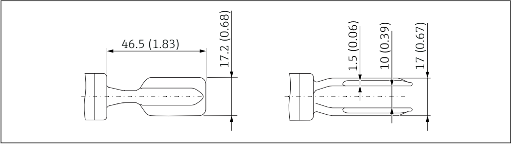
39 Tuning fork with enamel coating. Unit of measurement mm (in)
