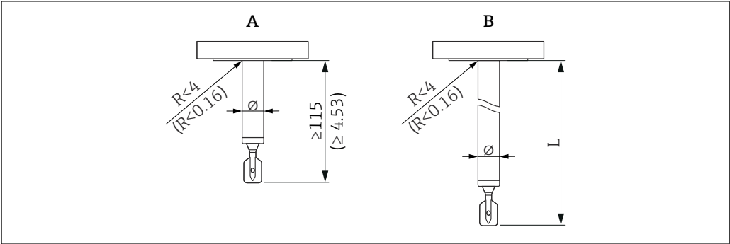
37 Probe design: short pipe, pipe extension. Unit of measurement mm (in)
