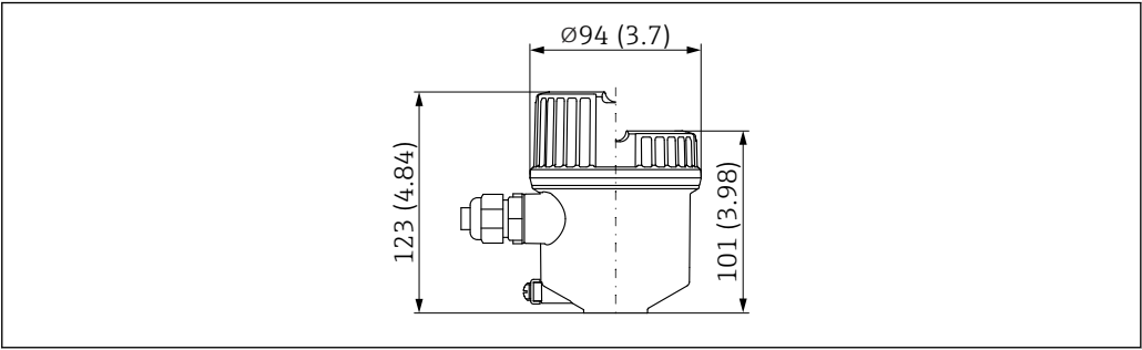
32 Single compartment; plastic housing. Unit of measurement mm (in)
