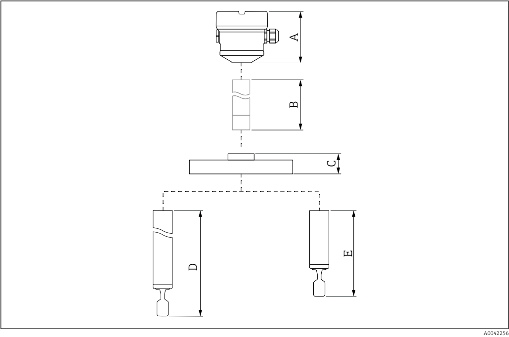
31 Components to determine the device height A Housing including cover B Temperature spacer, pressure-tight feedthrough (optional), details in the Product Configurator C Process connection (flange) D Pipe extension with tuning fork E Short pipe with tuning fork
