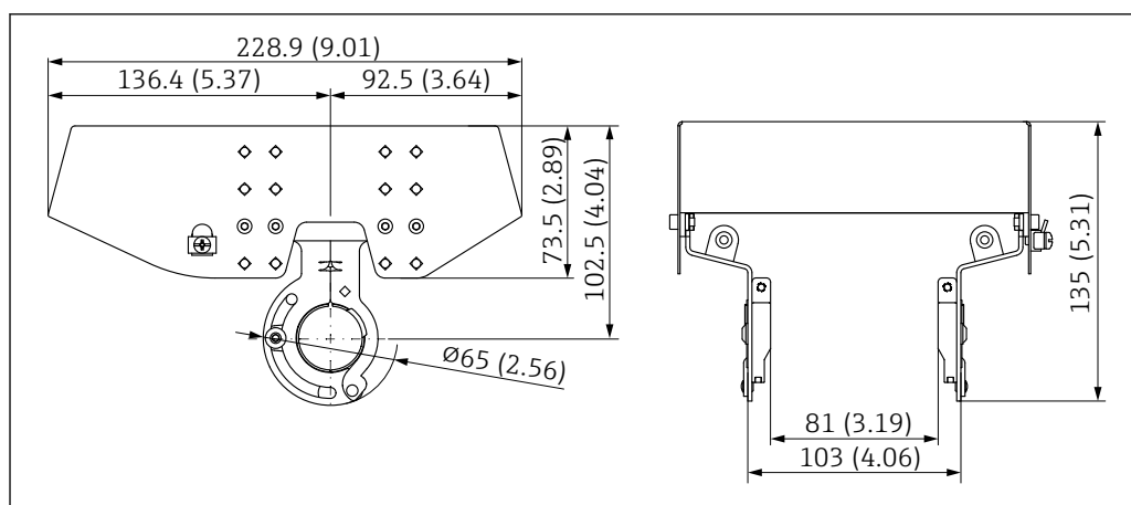
48 Weather protection cover for dual compartment housing, aluminum. Unit of measurement mm (in)
