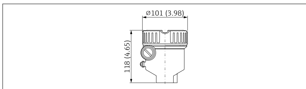
35 Single compartment; 316L, cast; also with Ex d/XP approval. Unit of measurement mm (in)
