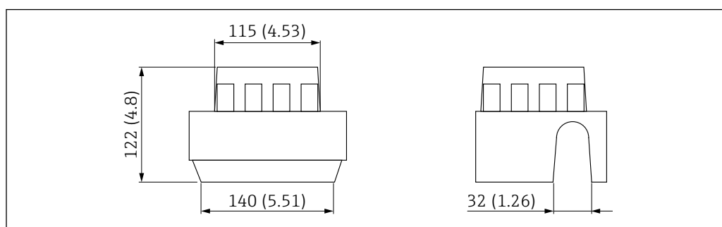
49 Protective cover for single compartment housing, aluminum or 316L. Unit of measurement mm (in)
