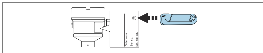
44 Functional test with test magnet
