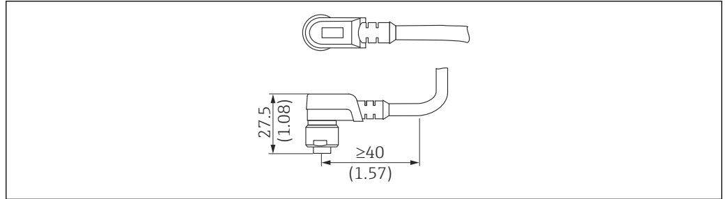
51 Plug-in jack M12 IP67. Unit of measurement mm (in)
