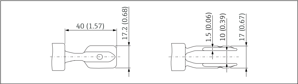
38 Tuning fork with plastic coating. Unit of measurement mm (in)
