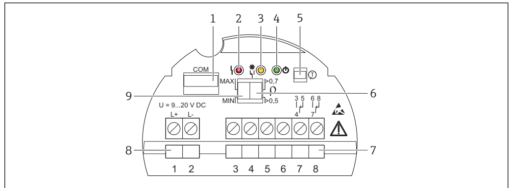
41 Example of electronic insert FEL64DC
