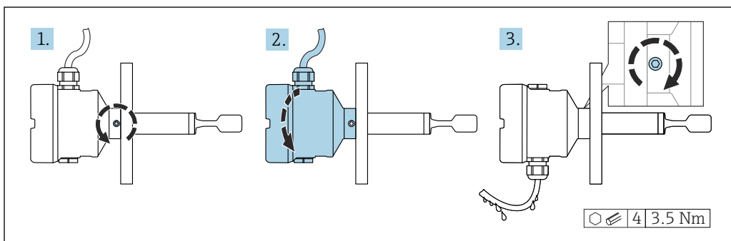
28 Housing with external locking screw and drip loop
