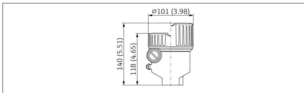
33 Single compartment; aluminum, coated; with Ex d/XP approval. Unit of measurement mm (in)
