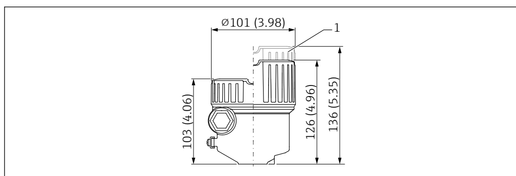
34 Single compartment; aluminum, coated. Unit of measurement mm (in)
