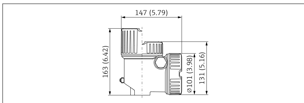
36 Dual compartment; L-shaped; aluminum, coated; also with Ex d/XP approval. Unit of measurement mm (in)
