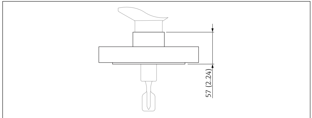
40 Process connection with flange
