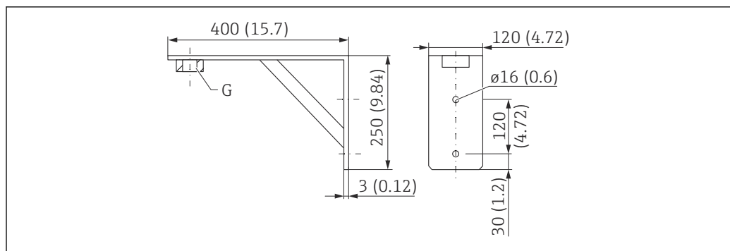
27 Dimensions of mounting bracket. Unit of measurement mm (in)
