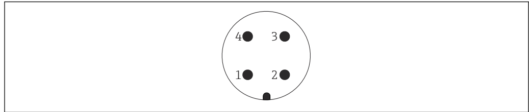
27 Pin assignment of M12 plug
