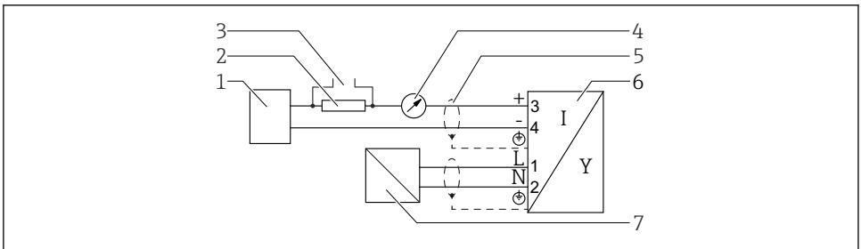
13 Blokdiagram, 4-draads: 4 ... 20 mA HART (90 ... 253 V AC )
