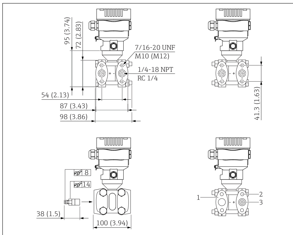
6 Front view, left-hand side view, right-hand side view. Unit of measurement mm (in)
