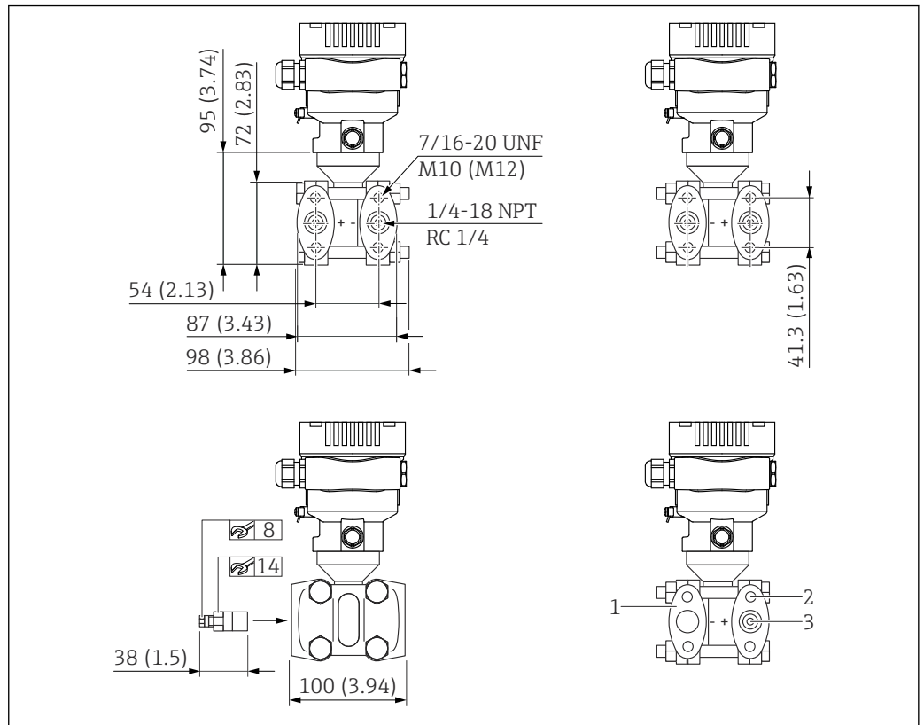
6 Front view, left-hand side view, right-hand side view. Unit of measurement mm (in)
