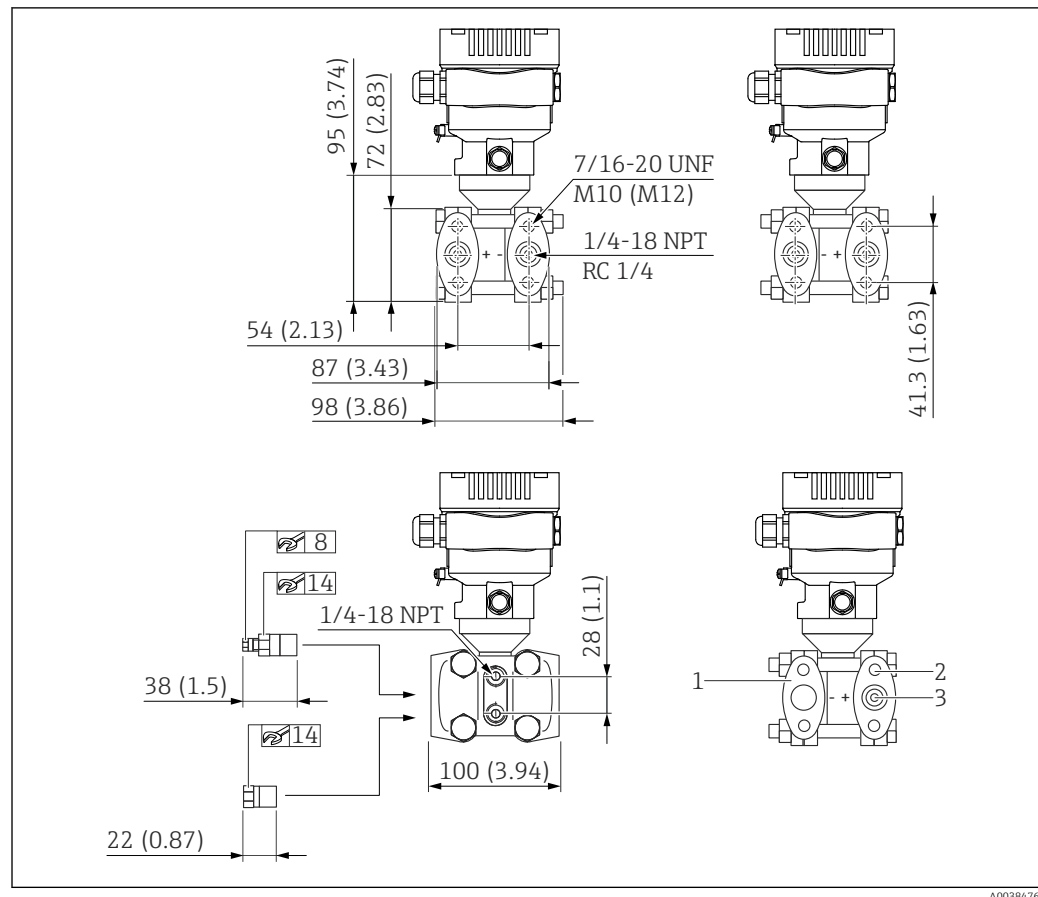
7 Front view, left-hand side view, right-hand side view. Nuts are always located on the minus side. Unit of measurement mm (in)
