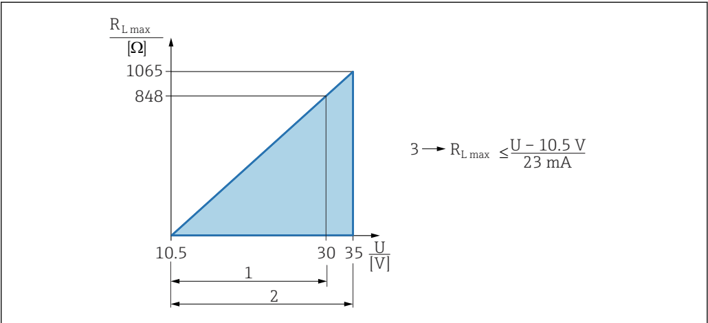
31 4 ... 20 mA HART 负载
