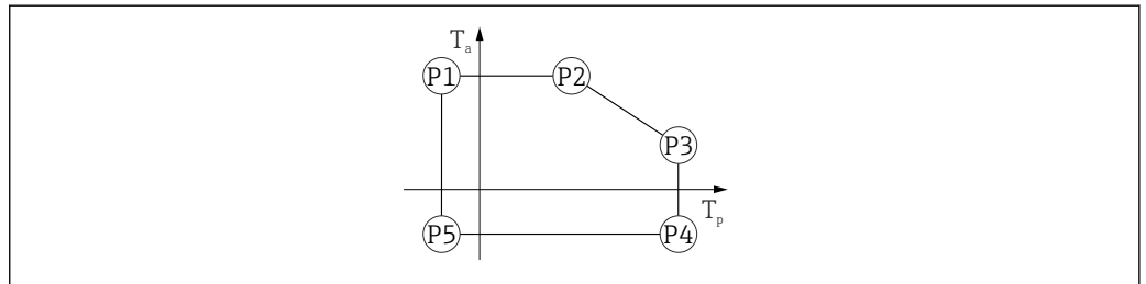
■ 31 铝外壳材质; 过程温度范围: -40 \dots +80 \text{ }^{\circ}\text{C} ( -40 \dots +176 \text{ }^{\circ}\text{F} )
