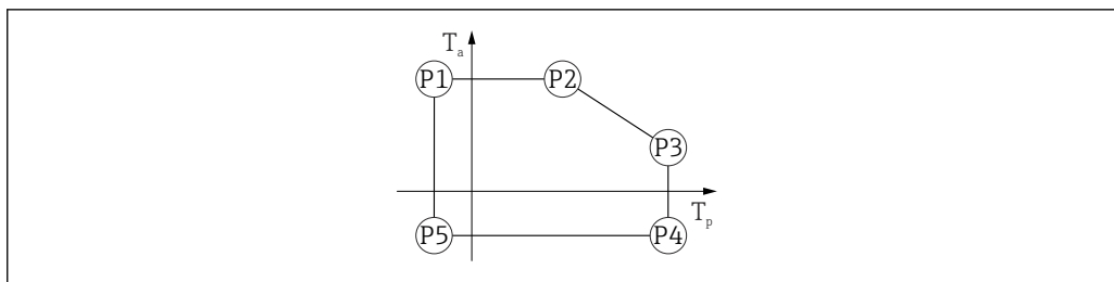
19 塑料外壳材质; 过程温度范围: -40 \dots +150\text{ }^{\circ}\text{C} ( -40 \dots +302\text{ }^{\circ}\text{F} )
