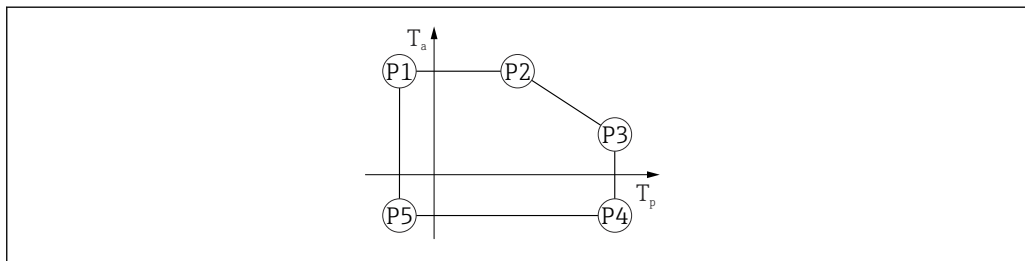
■ 25 铝外壳材质; 过程温度范围: -40 \dots +150 \text{ }^{\circ}\text{C} ( -40 \dots +302 \text{ }^{\circ}\text{F} )
