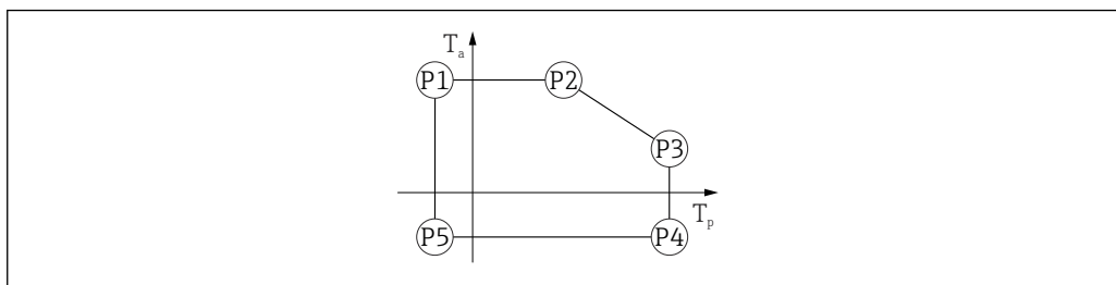
■ 26 铝外壳材质; 过程温度范围: -40 \dots +200 \text{ }^{\circ}\text{C} ( -40 \dots +392 \text{ }^{\circ}\text{F} )
