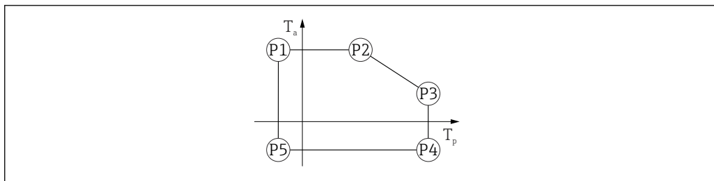
■ 24 铝外壳材质; 过程温度范围: -20 \dots +200 \text{ }^{\circ}\text{C} ( -4 \dots +392 \text{ }^{\circ}\text{F} )
