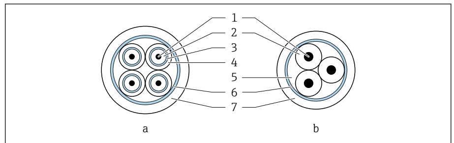
3 Cable cross-section
