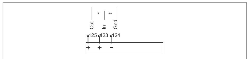
12 Assignment of the analog input
