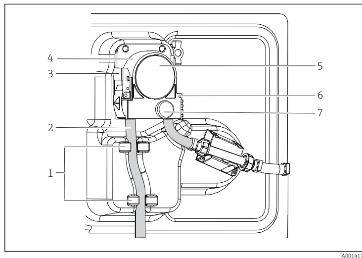
24 Opening the peristaltic pump
