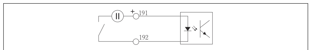
14 Binary input with external voltage source
