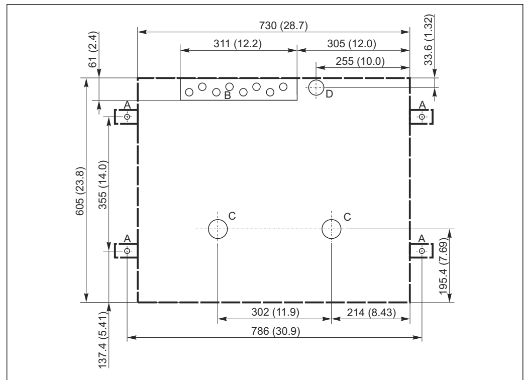
5 Foundation plan. Unit of measurement mm (in)
