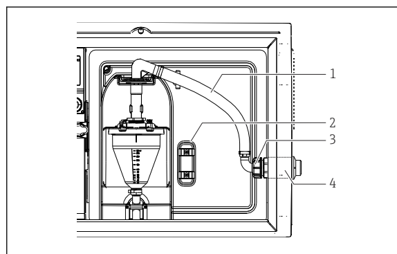
7 Connecting the suction line from the side (as-delivered state)
