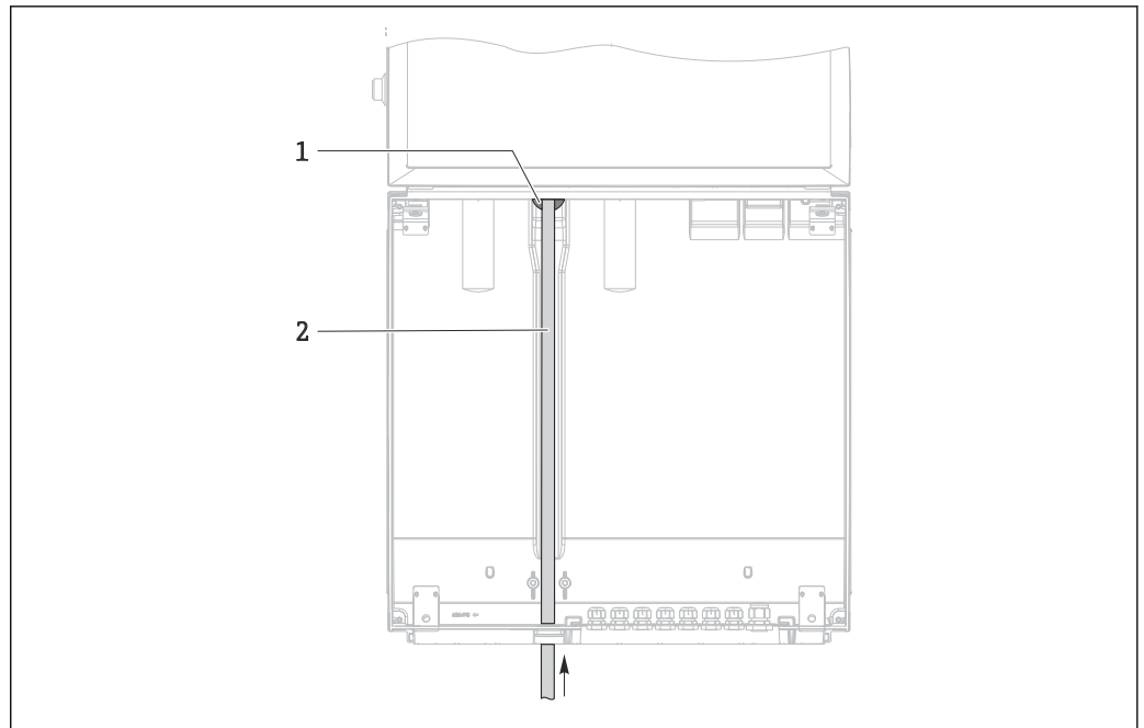
6 Sample supply from below
