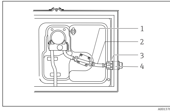
9 Connecting the suction line from the side (as-delivered state)
