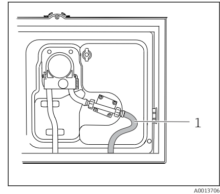
10 Suction line connected from below
