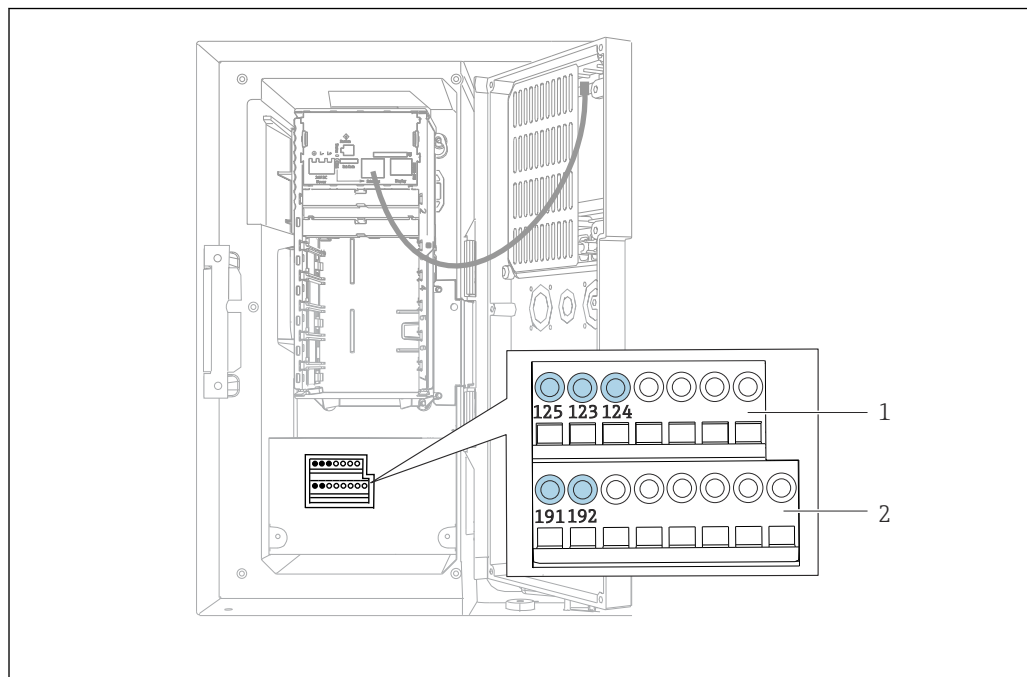
11 Interior of the controller housing
