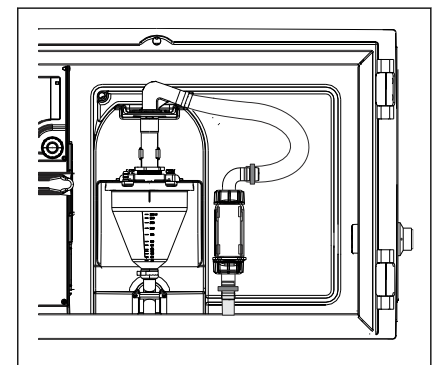
8 Suction line connected from below
