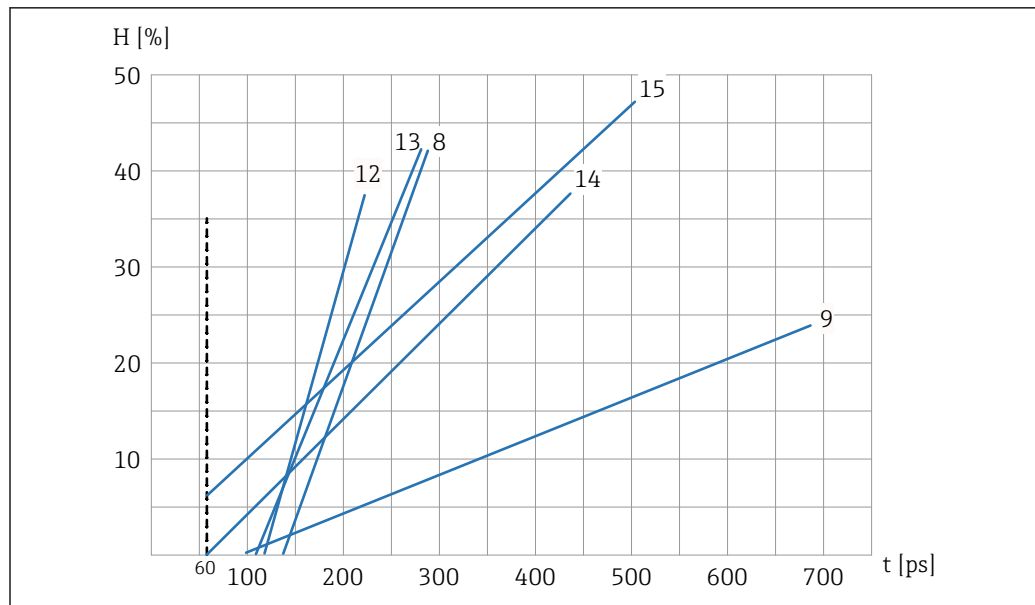
9 Ensemble de courbes d'étalonnage A (Cal.8, Cal.9, Cal.12, Cal.13, Cal.14, Cal.15)
