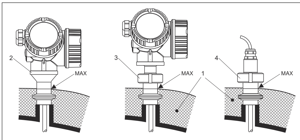
5 Raccords process hygiéniques - FMP53
