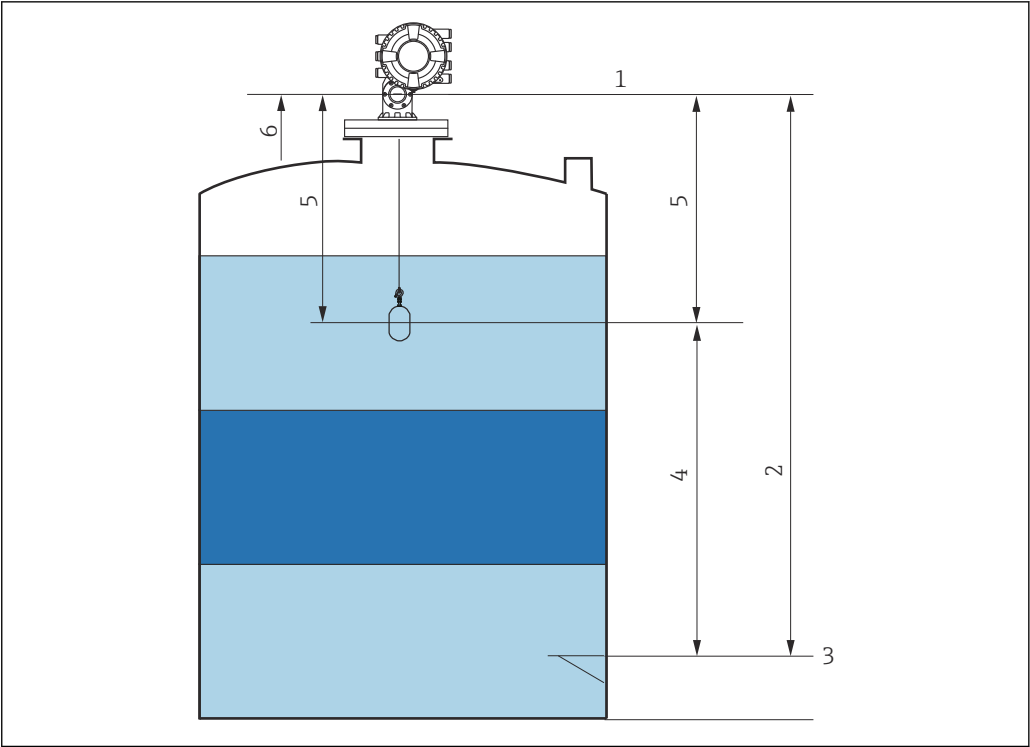
23 Displacer waiting for the liquid level to rise during standby level gauge command
