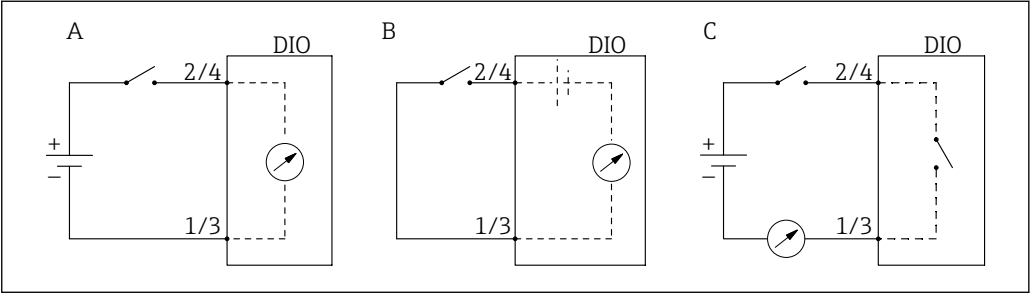
14 Operating modes of the Digital I/O module
