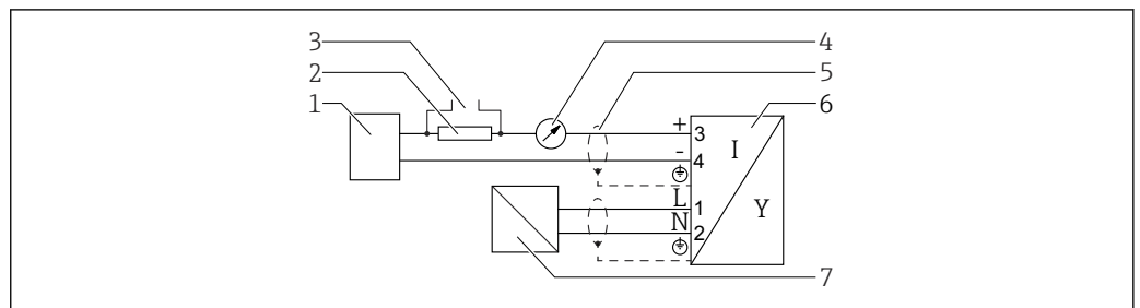
23 Blockdiagramm 4-Draht: 4 ... 20 mA HART (90 ... 253 V AC )
