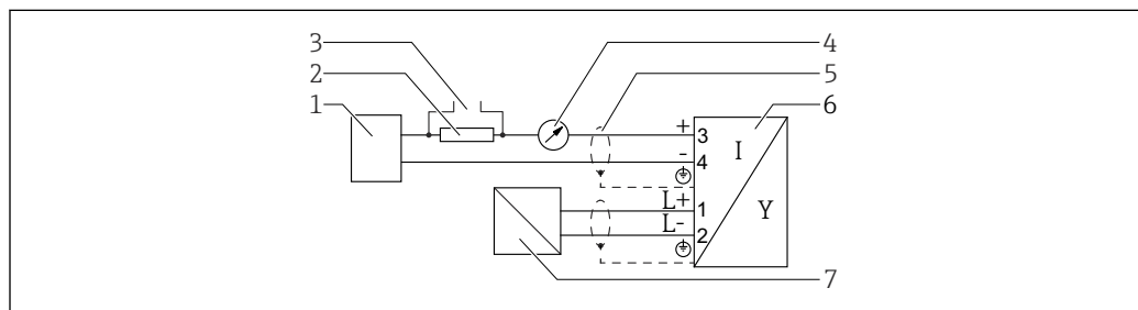
21 Blockdiagramm 4-Draht: 4 ... 20 mA HART (10,4 ... 48 V DC )
