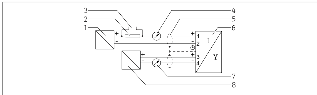
19 Blockdiagramm 2-Draht: 4 ... 20 mA HART, 4 ... 20 mA
