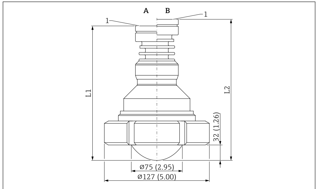
36 Dimensions of antenna, cladded flush mount, PTFE, 80 mm (3 in), slotted nut DIN11851. Unit of measurement mm (in)
