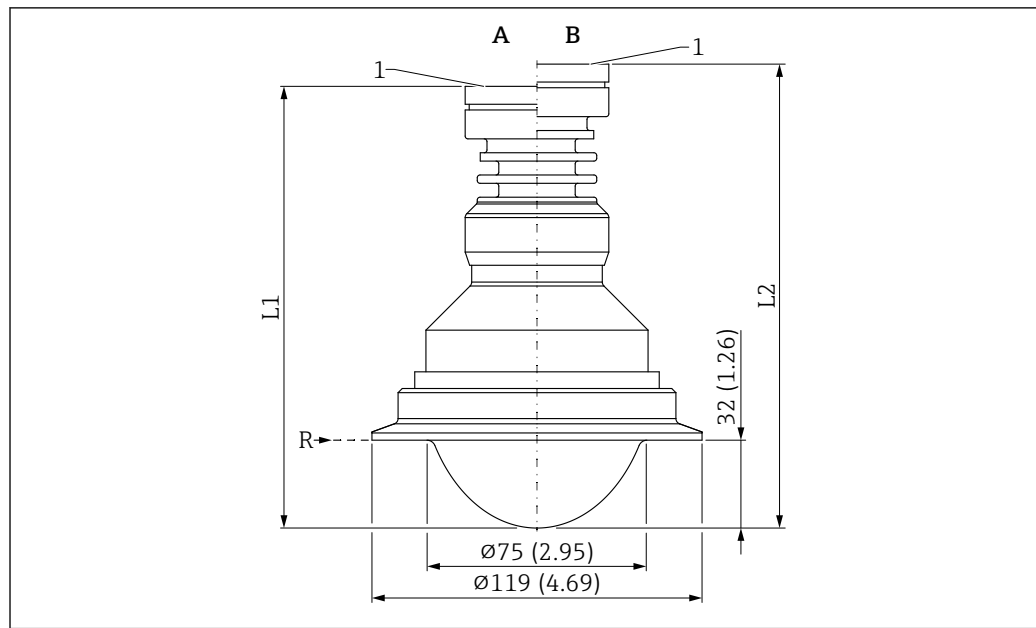
39 Dimensions of antenna, cladded flush mount, PTFE, 80 mm (3 in), with Tri-Clamp DN101.6 (4") ISO2852. Unit of measurement mm (in)
