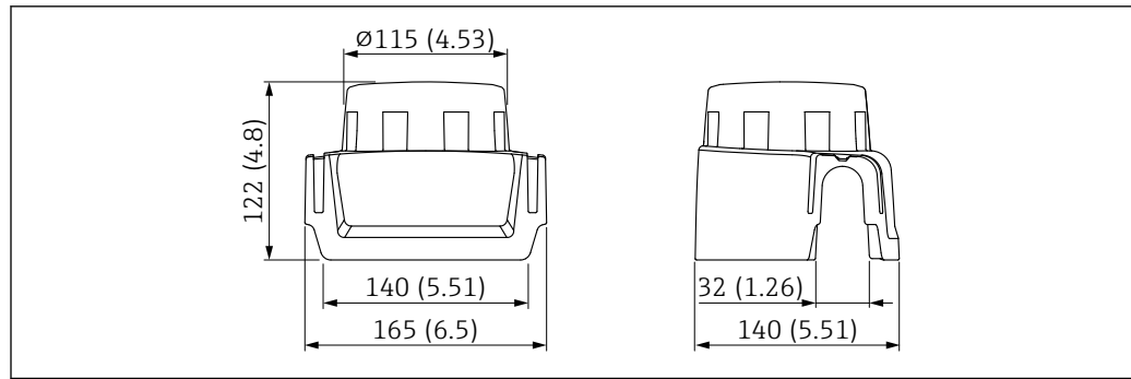
48 Dimensions. Unit of measurement mm (in)
