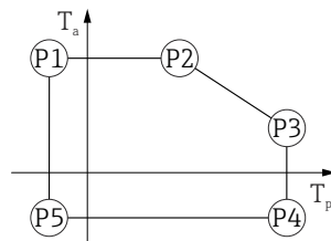
25 316L housing, hygiene; process temperature -20 to +150 °C ( -4 to +302 °F)
