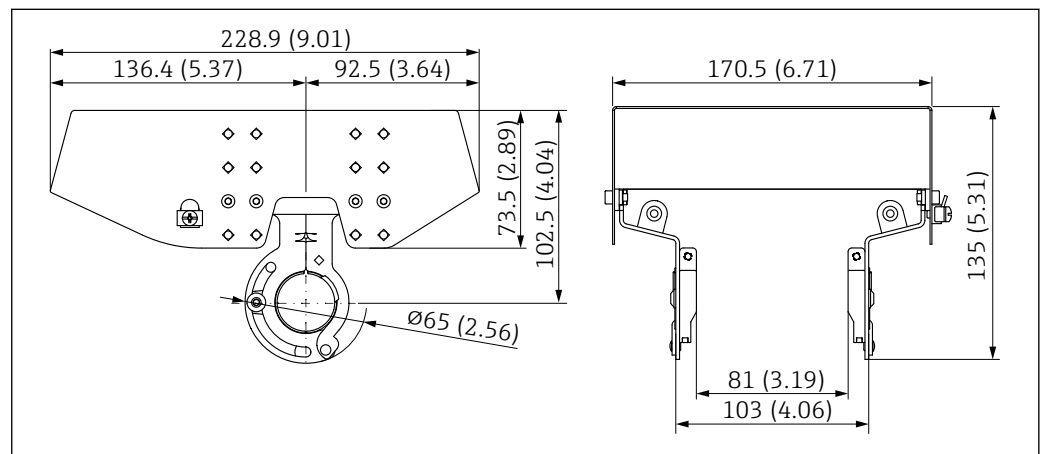
47 Dimensions. Unit of measurement mm (in)
