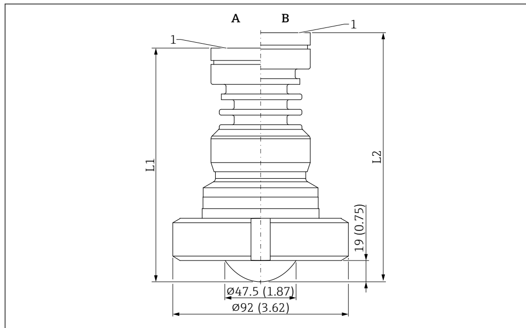
35 Dimensions of antenna, cladded flush mount, PTFE, 50 mm (2 in), slotted nut DIN11851. Unit of measurement mm (in)
