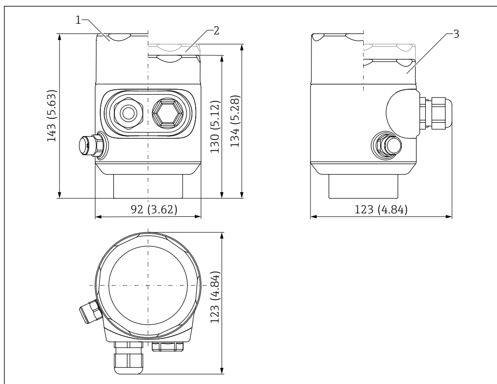
31 Dimensions of single compartment housing, 316L, hygiene. Unit of measurement mm (in)
