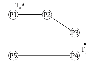
27 316L housing, hygiene; process temperature range: -40 to +150 °C ( -40 to +302 °F)
