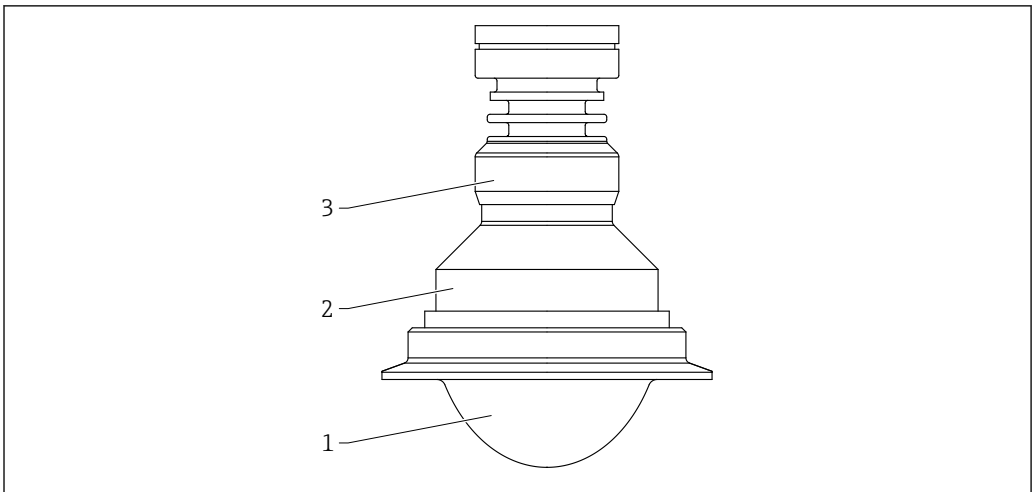
44 Material; antenna, cladded flush mount, PTFE, 80 mm (3 in), with Tri-Clamp ISO2852
