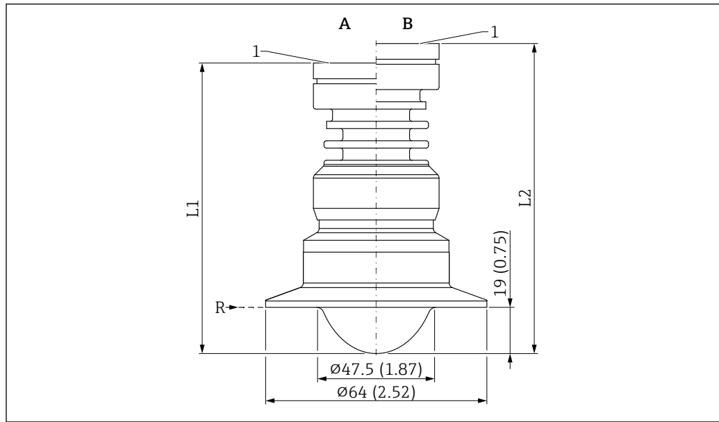
37 Dimensions of antenna, cladded flush mount, PTFE, 50 mm (2 in), with Tri-Clamp DN51 (2") ISO2852. Unit of measurement mm (in)
