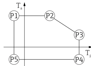
28 316L housing, hygiene; process temperature -40 to +200 °C ( -40 to +392 °F)
