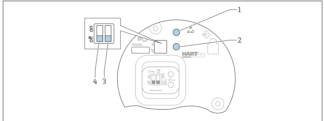
45 Operating keys and DIP switches on the HART electronic insert
