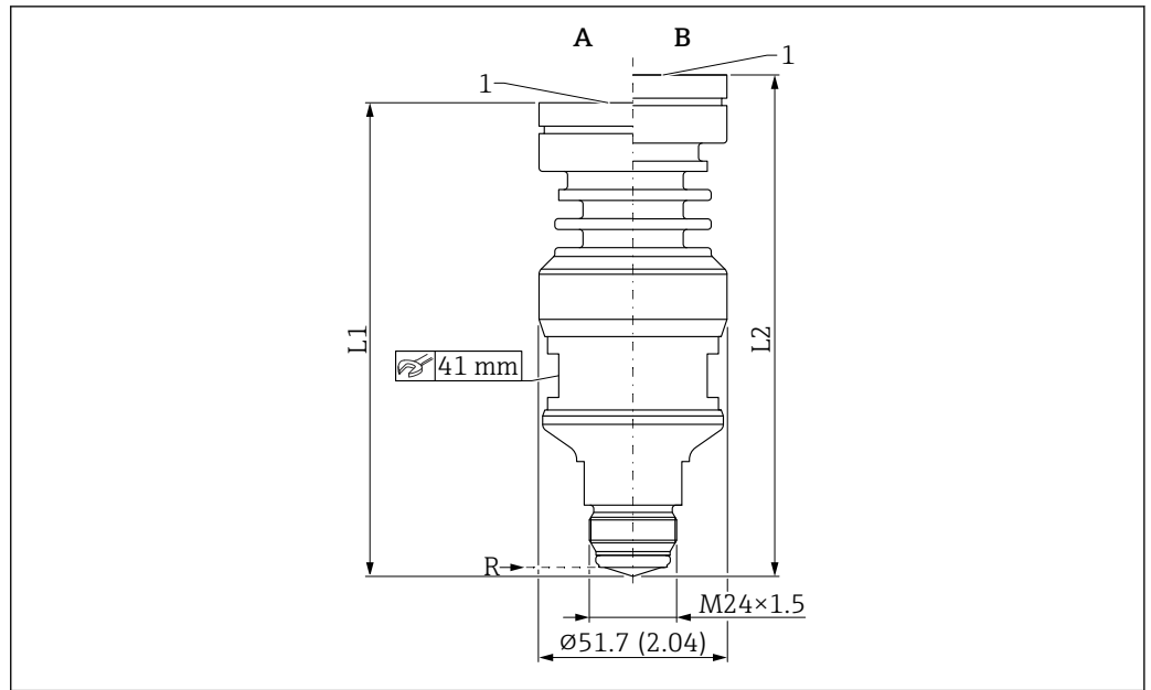
34 Dimensions of integrated antenna, PEEK, 20 mm / M24×1.5. Unit of measurement mm (in)
