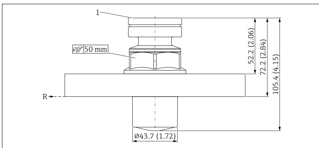
47 Dimensions of encapsulated antenna, PVDF, 40 mm (1.5 in), process connection UNI flange. Unit of measurement mm (in)
