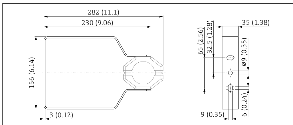
68 Dimensions of mounting bracket. Unit of measurement mm (in)
