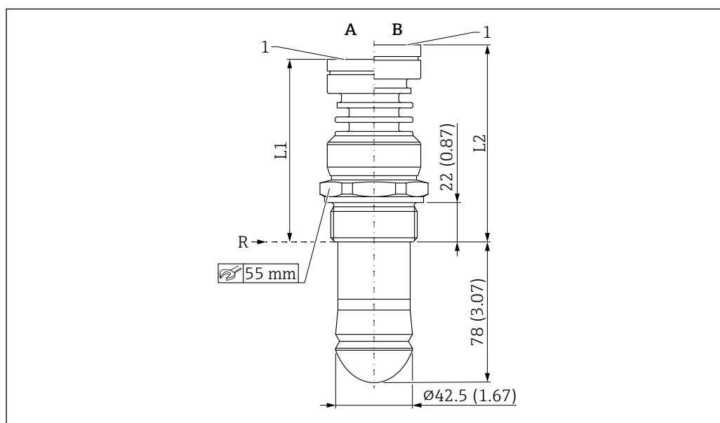
51 Dimensions of Drip-off antenna 50 mm (2 in), threaded process connection. Unit of measurement mm (in)
