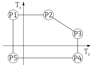
33 316L housing; process temperature range: -40 to +150 °C ( -40 to +302 °F)
