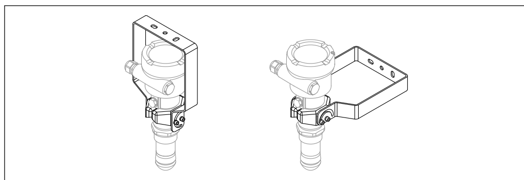
42 Ceiling or wall mounting
