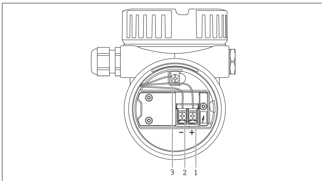
5 Connection terminals and ground terminal in the connection compartment
