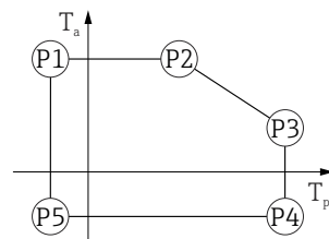
19 316L housing, hygiene; process temperature -40 to +130 °C ( -40 to +266 °F)
