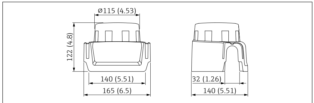
41 Dimensions. Unit of measurement mm (in)
