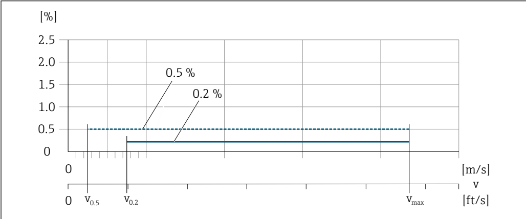
41 Flat Spec in % v.i.
