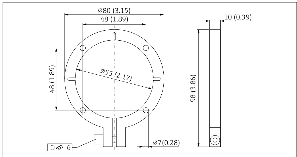
24 Mounting flange, 1.4301, for rod sensor
