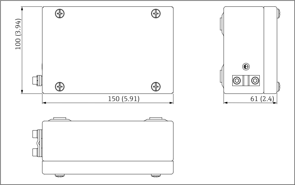
21 Dimension of ATEX electronics housing. Unit of measurement mm (in)
