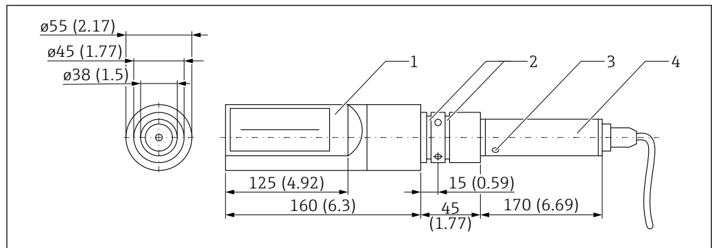
23 Dimensions of rod sensor. Unit of measurement mm (in)
