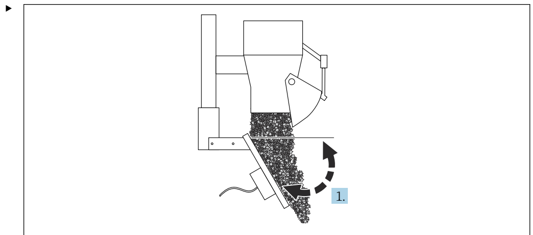
9 Abrasive bulk solids, positioning of baffle plate - opening hatch
