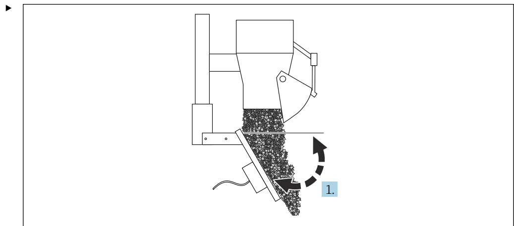
7 Abrasive bulk solids, positioning of baffle plate - opening hatch
