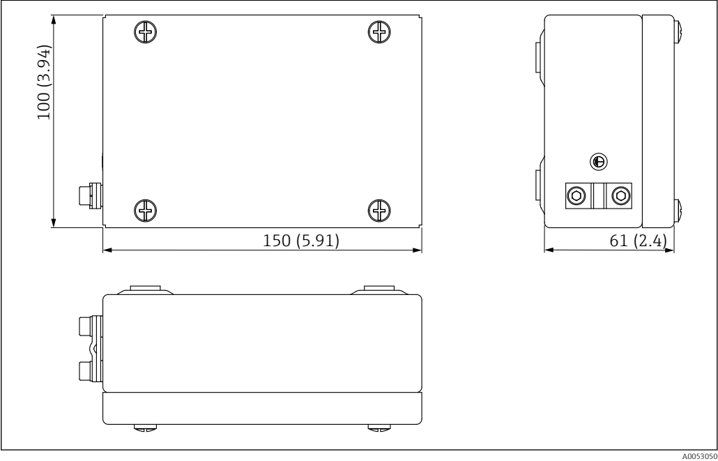
18 Dimension of ATEX electronics housing. Unit of measurement mm (in)
