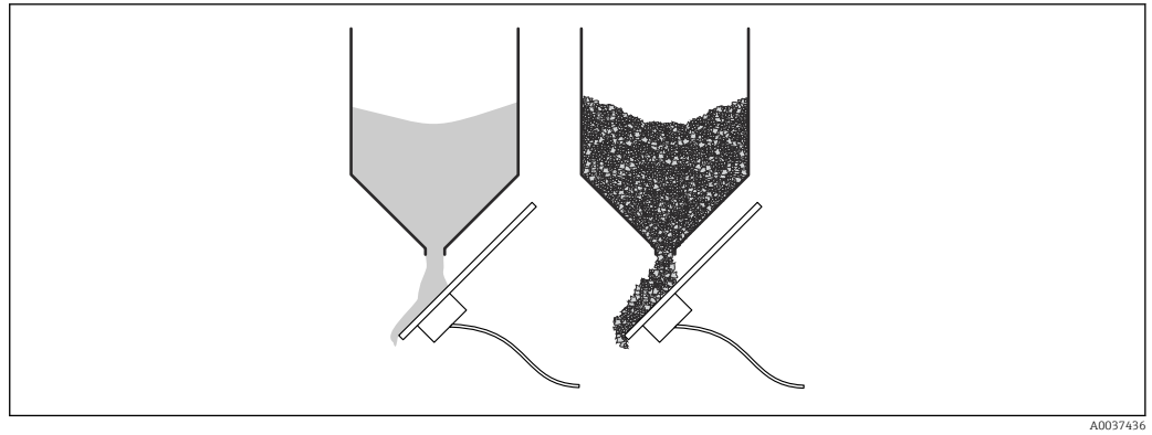
5 Installation of the round sensor for the measurement of bulk solids under silo discharge hatches
