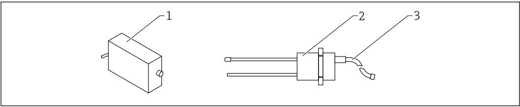
3 Rod sensor, ATEX version 1 ATEX electronics housing 2 Two-rod sensor, round design 3 Cable; UNITRONIC PUR CP
